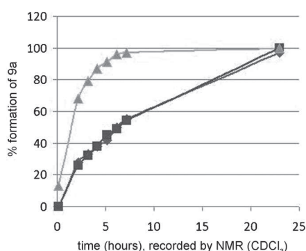
Figure 2. Kinetics of formation of 9a from 8a in various conditions. ♦ = TFA (7 equiv); ■ = TFA (7 equiv) + H 2 O (2 equiv); ▲ = TFA (20 equiv).
