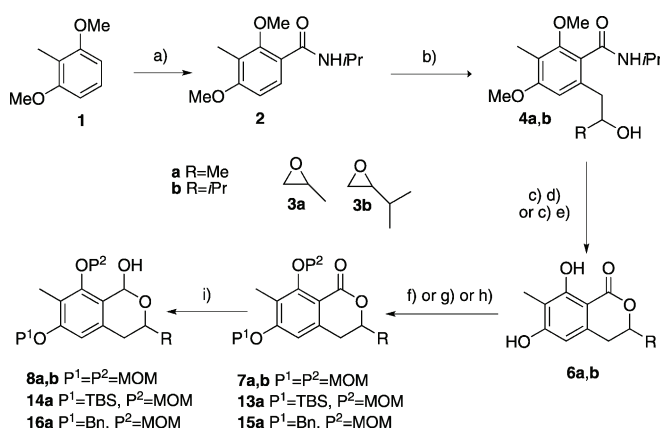
Scheme 2. Synthesis of lactols 8 , 14 , and 16 . Reaction conditions: a) i PrNCO, \text{AlCl}_3 , 95%; b) t BuLi/TMEDA then 3a or 3b ( 4a , 82%; 4b , 52%); c) CSA/toluene reflux; d) \text{AlCl}_3 ( 6a , 95%, 2 steps); e) \text{BBr}_3 ( 6b , 68%, 2 steps); f) NaH/MOMCl (2 equiv), ( 7a , 98; 7b , 91%); g) TBSCl/ \text{Et}_3\text{N} then NaH/MOMCl ( 13a , 89%); h) BnBr/ \text{K}_2\text{CO}_3 then NaH/MOMCl ( 15a , 83%); i) DIBAL-H, toluene, -78^\circ\text{C} .
