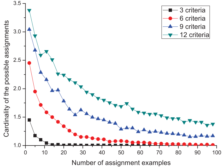
Figure 4.4: Cardinality of possible assignments versus the number of assignment examples: experiments to compute robust assignments of ELECTRE TRI models involving varied number of criteria, 4 categories.
