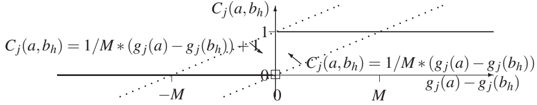
Figure 5.1: constraining C_j(a_e, b_h) to the appropriate value
