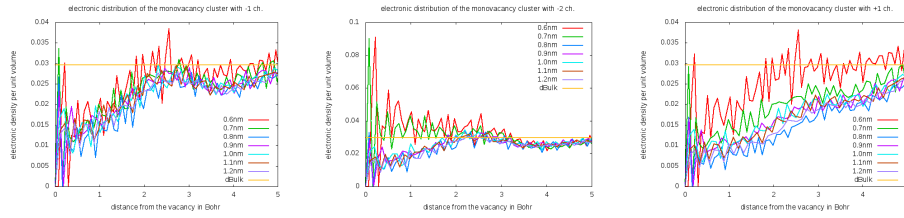
Figure 5.11: The variation of the electron density per unit volume around each shell of the nano cluster with a monovacancy (a) with 1 negative charge (b) with 2 negative charge (c) with 1 positive charge , around the vacancy.
