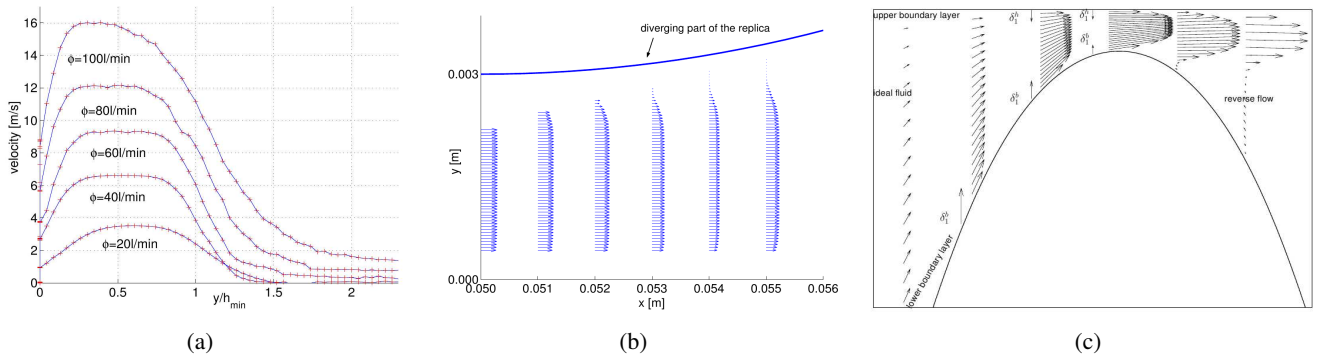
Figure 5.2: a) Measured vertical ( y -axis) velocity profile at 9mm downstream the minimum constriction of 2.3mm. Note the asymmetrical flow behaviour for \phi = 100 l/min. b) Measured bidimensional velocity profile illustrating jet formation and flow separation along diverging part of replica for steady flow of \phi = 40 l/min and minimum aperture 3mm. A step of 1mm is applied in the longitudinal x -direction and 0.05mm in the transverse y -direction. c) Reduced Navier Stokes (RNSP) computation ( Re_b = 500 ). The two upper and lower boundary layers and the ideal fluid appear from the computation. The interaction between the ideal fluid and the boundary layers is the core of the Interactive Boundary Layer theory [54].
