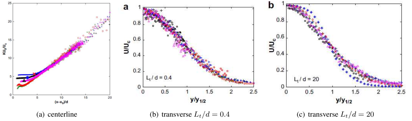
Figure 4.2: a) Inverse normalised longitudinal mean centerline velocities compensated for the self-similar law KU_0/U_c : L_t/d 0.4 ( \times ), 1.2 ( \circ ), 3.6 ( \triangle ), 7.2 ( + ) and 20 ( \triangleright ). The potential core x_p in the self-similar representation is indicated for L_t/d 3.6 ( \triangle ), 7.2 ( * ) and 20 ( \triangleright ) and b,c) Similarity representation of transverse normalised axial mean velocity profiles U/U_c for x/d 1.6 ( \star ), 3.2 ( \diamond ), 4 ( + ), 4.8 ( \times ), 6.4 ( \circ ), 8 ( \triangleright ), 12 ( \triangle ), 16 ( \square ).
