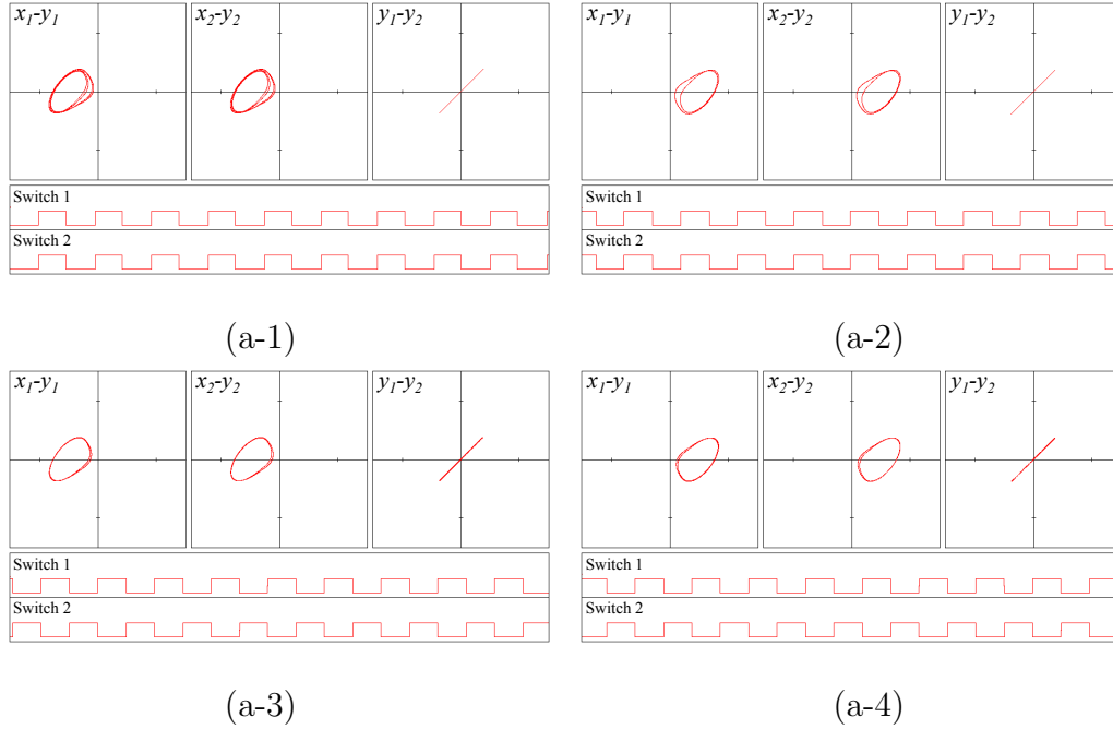
Figure 5.3 Attractors and phase differences in the coupled parametrically forced Chua's circuit. (a) r = 4.0 . (b) r = 6.0 .
