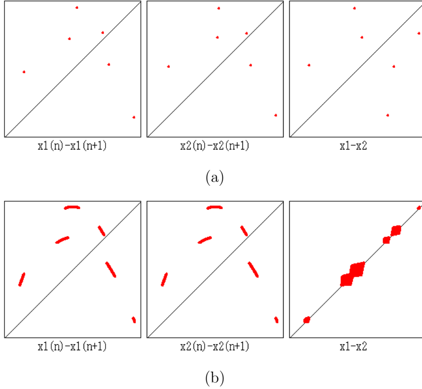
Figure 3.6 return maps and phase differences in coexistence of period six orbit and chaotic orbit depending on initial values. \alpha_1 = 2.94 , \alpha_2 = 3.84 and \varepsilon = 0.04 .
