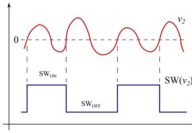
Figure 4.2 The motion of the switch depending on v_2 .
