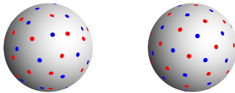
Figure 8.6: (left) incrementally constructed point set on S = 2 shells, K_s = 17 points per shell, and (right) optimal configuration for the same parameters. For such a small sample size, the incremental construction gives poorly uniform configurations.
