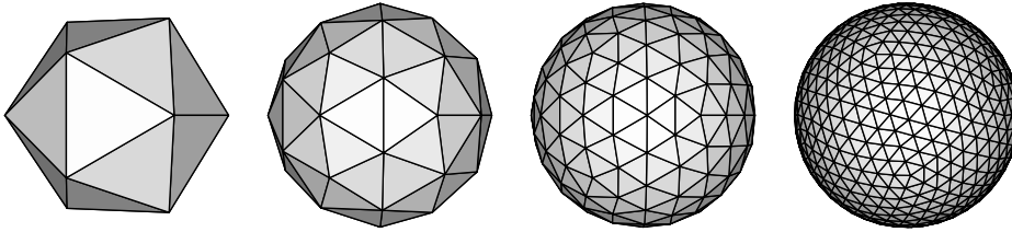
Figure 5.2: Sphere tessellation from an icosahedron. From left to right: regular icosahedron (12 vertices), two-fold tessellated icosahedron (42 vertices), 4-fold tessellated icosahedron (162 vertices) and 8-fold tessellated icosahedron (642 vertices).
