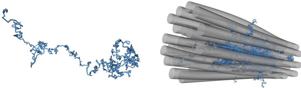
Figure 3.5: (left) Free Brownian motion of a water molecules. (right) A bundle of white matter fibers, and water molecules trajectory within. We simulated here a bundle of 19 fibers, each fiber has a 5\ \mu\text{m} radius, and we observe the trajectory of 100 water molecules, over 60 ms.
