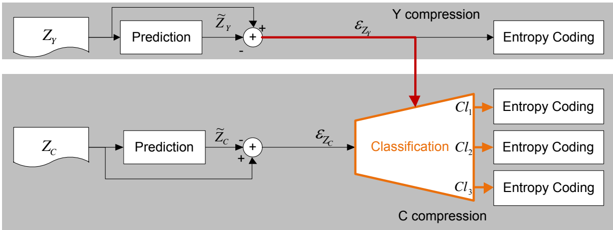
Figure 3.2: Multi component classification scheme
