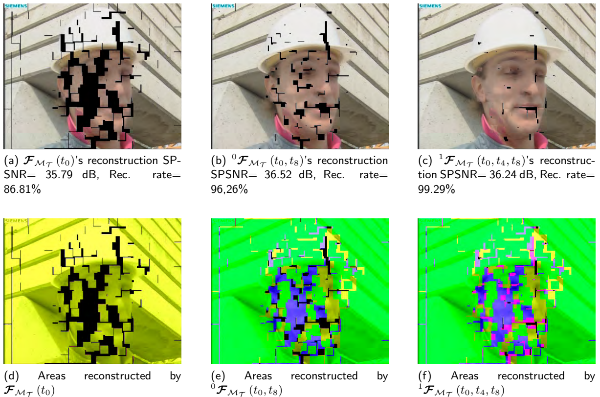
Figure 6.20: B-families of motion tubes: influence on the synthesis of the fourth image of sequence Foreman
