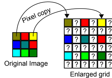
Figure 5.4: Step 1 - Pixel copy over an enlarged grid
