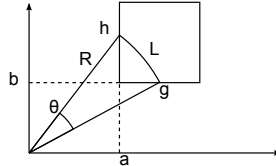
Figure 6.23: Descriptor Integral on a discrete array.
