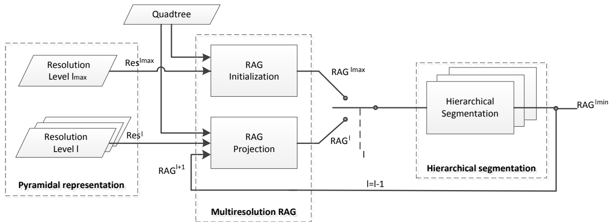
Figure 5.16: JHMS general scheme
