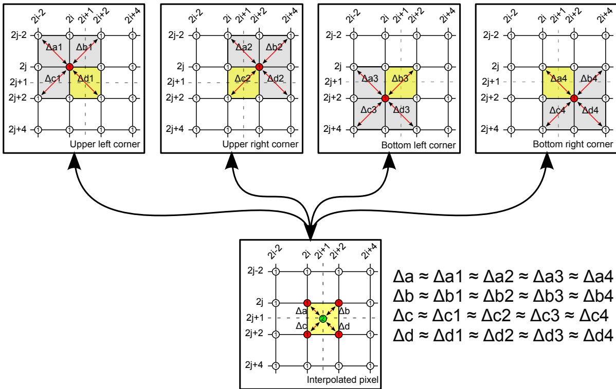
Figure 5.5: Step 2 - diagonal interpolation
