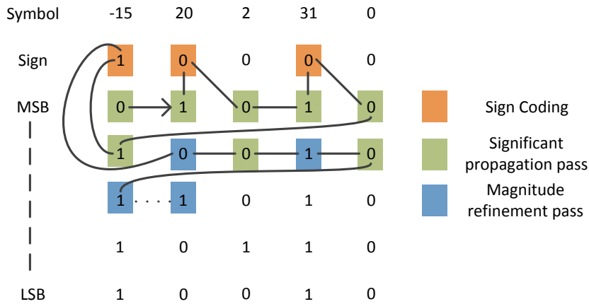
Figure 3.9: Example of QM coding with bit plane orientation
