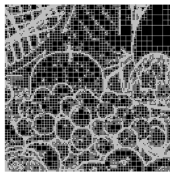
(b) Quadtree
