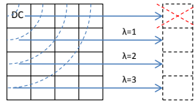
Figure 6.22: Descriptor computed on a 4x4 DCT block.
