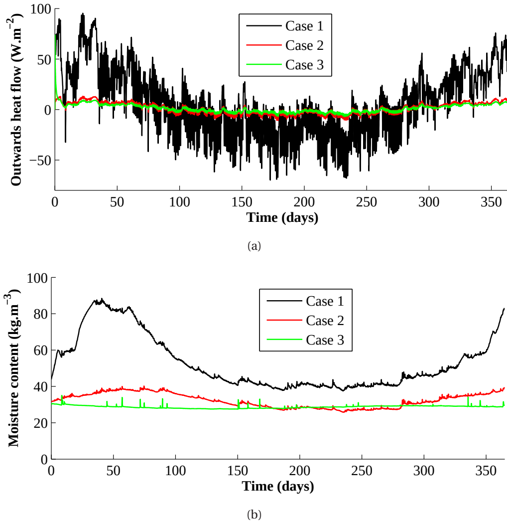
Figure 5.11: Effect of the facade orientation on the (a) outwards heat flow and (b) moisture content during a year of simulations
