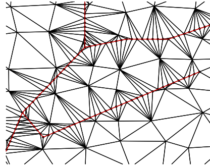
Figure 4.20: Close-up of the mesh resulting from a crack discretisation of 1 \times 10^{-4} m
