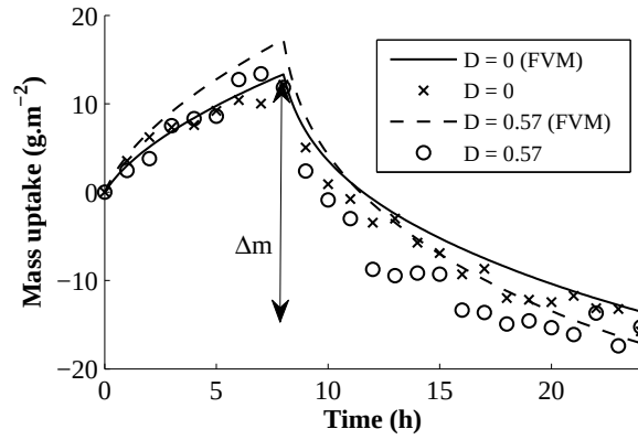
Figure 2.9: Mass measurements during one day of the Nordtest program and corresponding profiles computed by finite volume simulations
