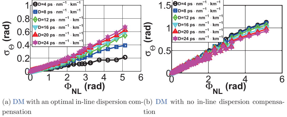
Figure 4.8: Curves of \sigma_{\Theta} as a function of the system cumulative \Phi_{NL} for an optimal dispersion management without optical filtering. The system parameters were varied following the table of figure 4.2. After fixing a value for the chromatic dispersion D , the optimization was separately achieved for each couple of values (P_{in}, N_{spans}) , choosing the lowest \sigma_{\Theta} for the variable parameters D_{lin} (for figure (a)), D_{pre} and D_{res} .
