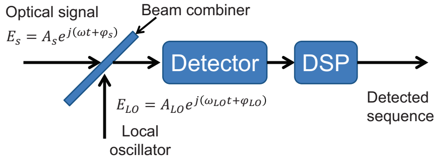
Figure 2.35: Coherent detection principle
