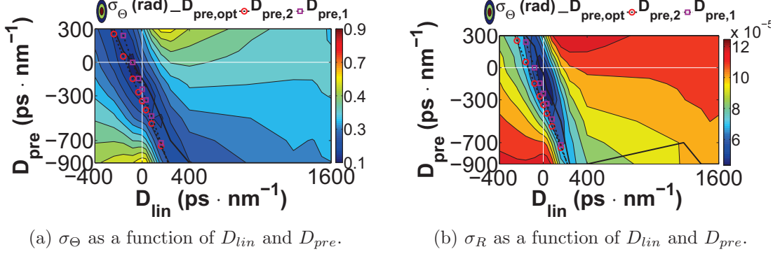
Figure 4.15: \sigma_\Theta and \sigma_R plotted as a function of D_{lin} and D_{pre} . System parameters: D = 16 \text{ ps} \cdot \text{nm}^{-1} \cdot \text{km}^{-1} , P_{in} = 9 \text{ dBm} , N_s = 6 , D_{res} = 0 \text{ ps} \cdot \text{nm}^{-1} , D_{pre} varying from -900 to 300 \text{ ps} \cdot \text{nm}^{-1} and D_{lin} varying from -400 up to 1600 \text{ ps} \cdot \text{nm}^{-1} . With a solid line the true minimum \sigma_R , with round markers the law of [43] and with square markers the law of [67]. Optical 2 nd order Gaussian filtering was performed before the receiver.
