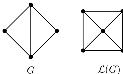
Figure 2.14: A graph and its line graph.
