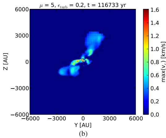
Fig. 10. Maximum of the projected radial velocity for \mu = 5 , for \epsilon_{\text{turb}} = 0.2 .
