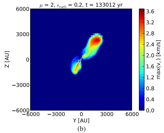
Fig. 11. Maximum of the projected radial velocity for \mu = 2 , for \epsilon_{\text{turb}} = 0.2 .
