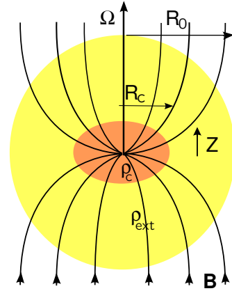
Fig. 2. Schematic view of a collapsing core in aligned configuration with field lines that fan-out. B is the magnetic field, R_c the radius of the core, R_0 the initial radius, Z the half-height of the transition region, \rho_c the density of the core, and \rho_{\text{ext}} the density of the external medium.
