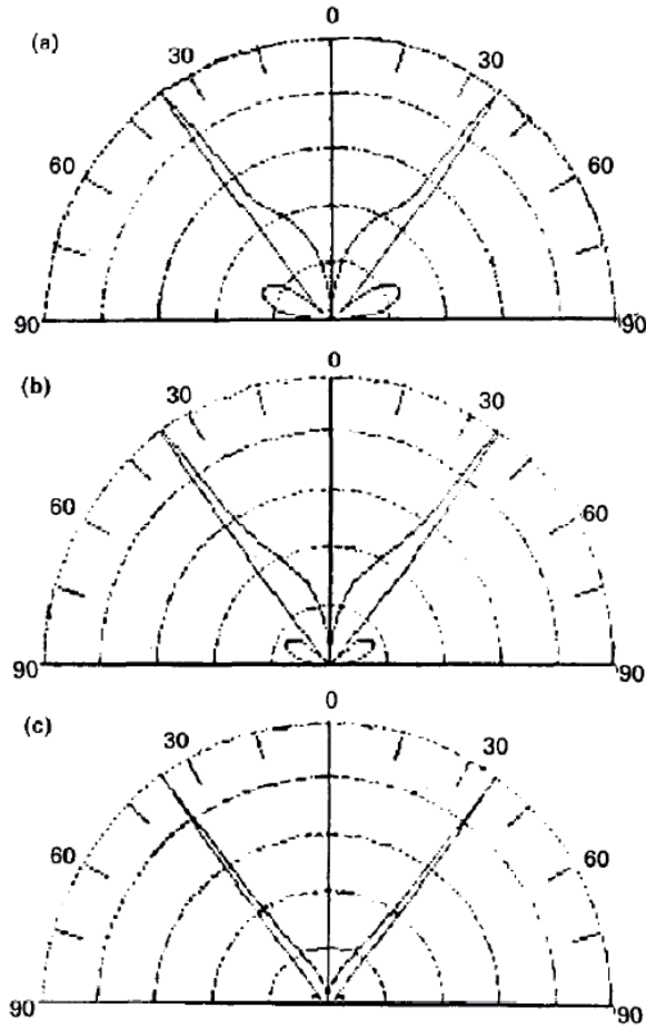
Figure 10 The directivity patterns of shear wave for three values of k_2/b , k_2a \ll 1 and Poisson's ratio \sigma=0.23 . k_2/b are, respectively (a) 0.01; (b) 1; (c) 6.28
