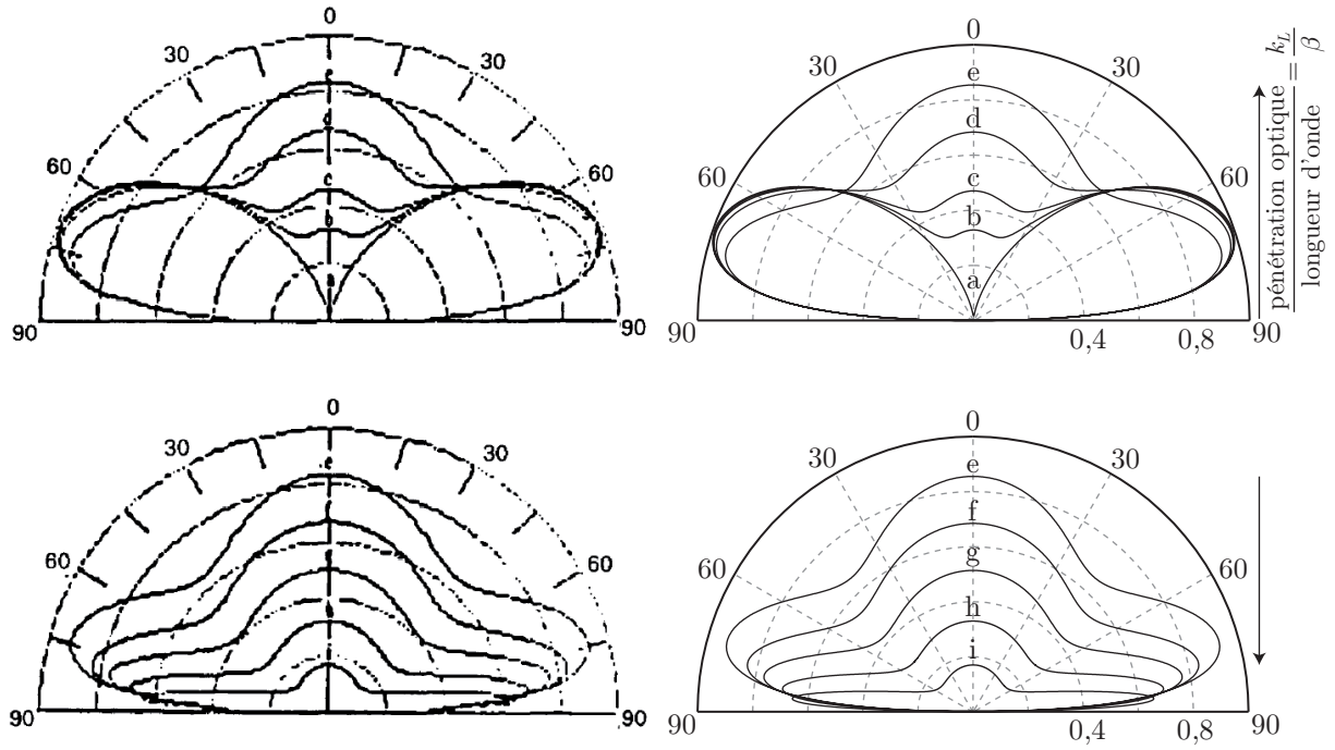
Figure 9 Variation of the longitudinal directivity pattern with k_L/b for k_1 \ll 1 and Poisson's ratio \sigma = 0.23 . k_L/b are, respectively, (a) 0.01; (b) 0.2; (c) 0.3; (d) 0.5; (e) 1, (f) 2; (g) 3; (h) 5; (i) 10
