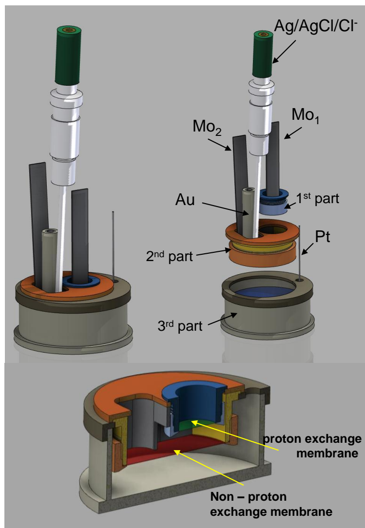
Fig. VI. 2. Schematics of the electrochemical cell.
