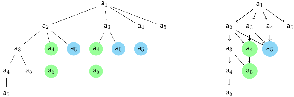
Figure 5.3: CTREE and CDAG storing chains of d_2
