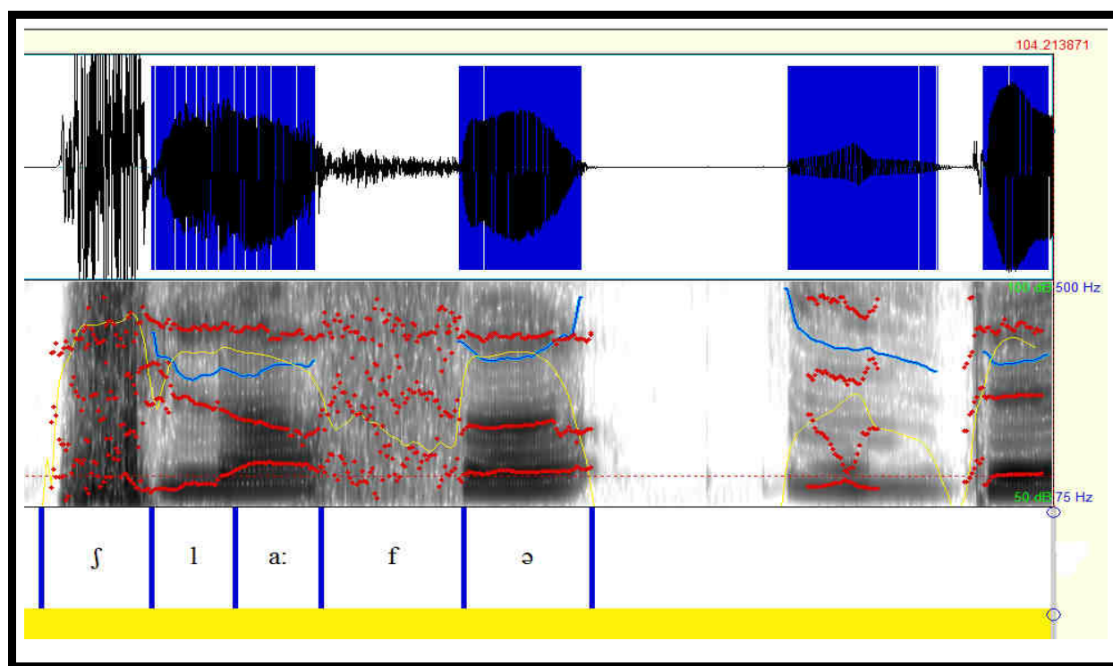
Figure 145 : LB, /lɑ:fə/ Test 1
