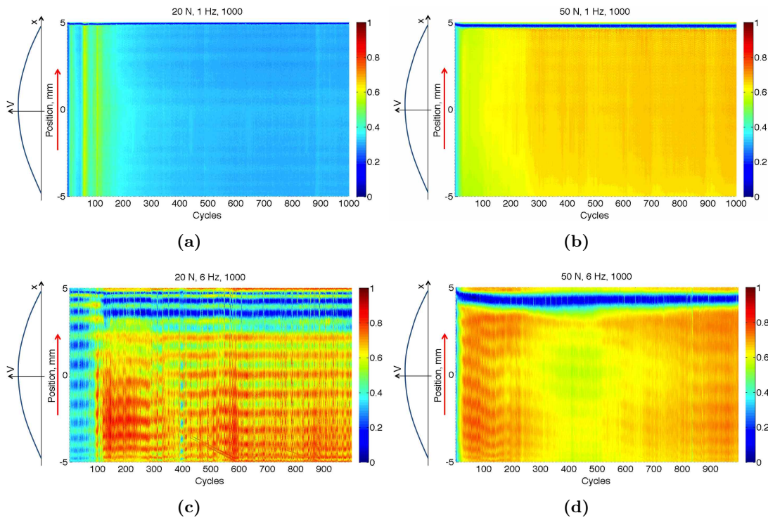
Figure 5.23: Friction maps for (a) 20 mm/s, 20 N; (b) 20 mm/s, 50 N, (c) 120 mm/s, 20 N, (d) 120 mm/s, 50 N of mean sliding velocity and normal force, respectively. The friction coefficient is averaged between back and forth passes for each cycle. The sliding distance on y -axis and cycle numbers on x -axis are limited by 10 mm and 1000 cycles, respectively
