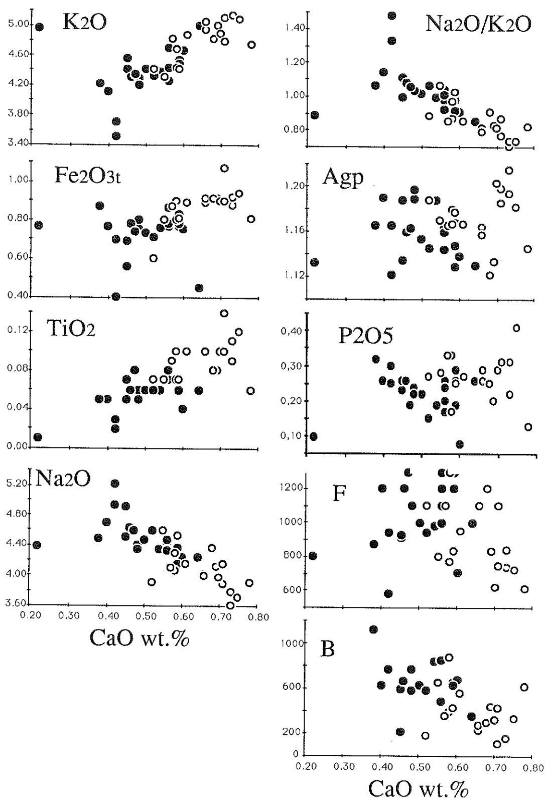
Fig. 58: Harker variations diagrams for the major elements. See text for explanations. Contents are in wt.% except for B and F which are in ppm. Same symbols as in Fig. 51.
