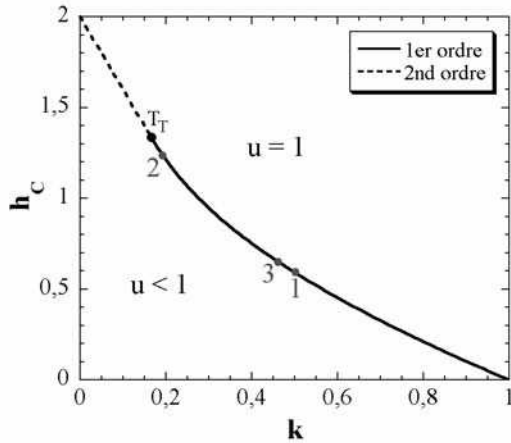
Figure 56: Diagramme de phases h_C = f(k) .
