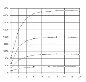
Rationnels/Flottants
