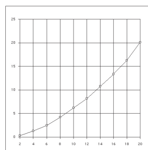
Flottants
