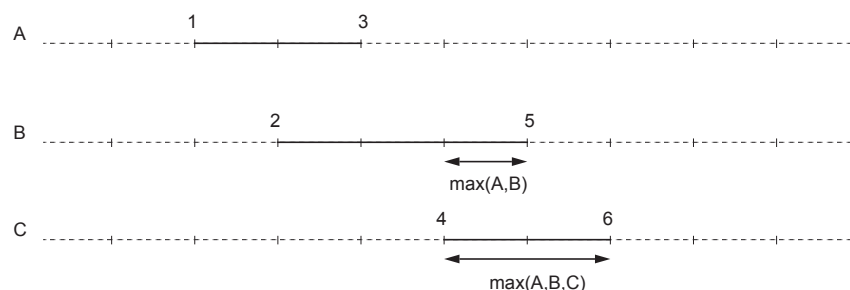
figure 36 Maximum paresseux
