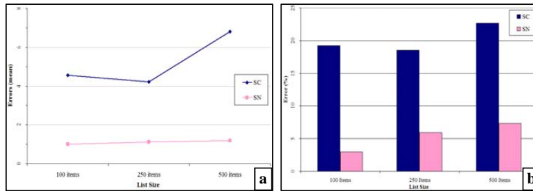
Fig. 7. Mean of errors (a) and Percentage of faulty trials (b) by Technique and by List Size
