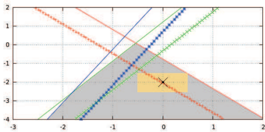
Figure 3.3: Satisfiable example without case-split analysis: model calculation
