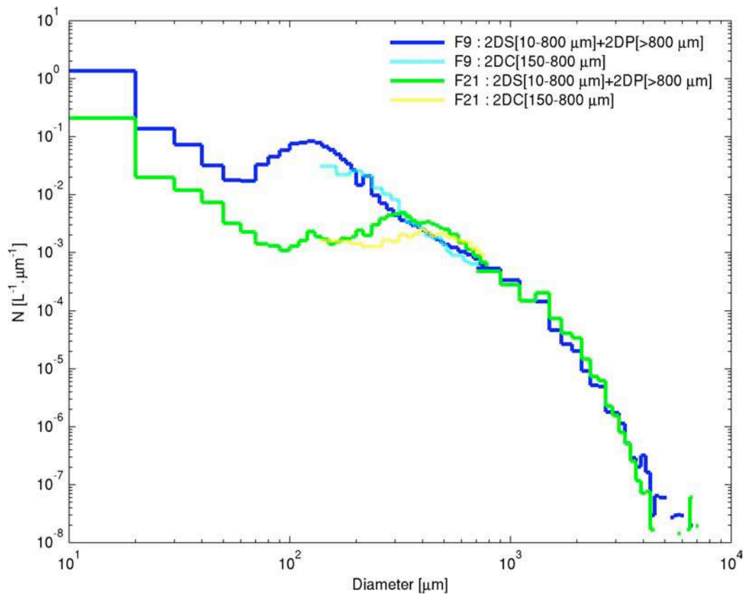
Figure 2.9 Averaged size distributions from 2DS, 2DC and 2DP probes for F9 (1 April 2008) in the time interval 23:13:43-23:32:10 UTC (in blue line) and for F21 (15 April 2008) in the time interval 00:55:26-01:14:58 UTC (in green line).
