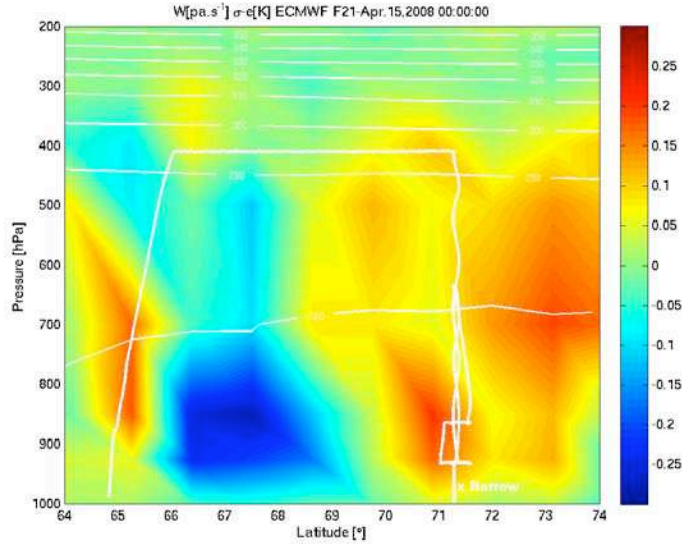
Figure 2.8 Vertical profile of flight F21 (in white full line) with equivalent potential temperature (K) and vertical velocity ( \text{Pa}\cdot\text{s}^{-1} ) over Alaska at 00:00:00 UTC (15 April 2008).
