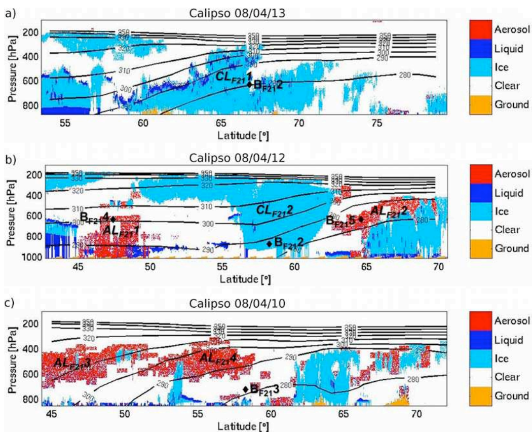
Figure 3.13 Dardar Mask track section observed on 13 April (a) at 23:01:00 UTC, on 12 April (b) at 14:18:00 UTC that intercept the FLEXPART air masses ( B_{F212} ) in positions ( \diamond ), and on 10 April at 13:00:00 UTC that intercept the FLEXPART air masses ( B_{F213} ) in positions ( \diamond ).
