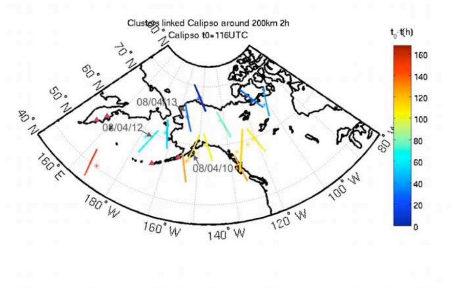
Figure 3.12 Calipso track sections (line) and FLEXPART air mass positions (*) along FLEXPART trajectories initialized in the box B_{F212} of Figure 3.11c (left of the dashed line) and initialized in the box B_{F213} of Figure 3.11e (right of the dashed line). The color scale indicates the elapsed time in hours between the CALIPSO observation and the aircraft observation.
