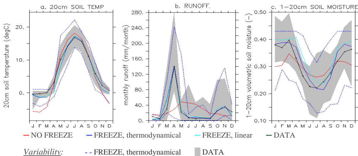
Figure 2.6. Annual cycles of monthly mean 20 cm soil temperature (a.), monthly mean runoff (b.) and monthly mean 1-20 cm soil moisture (c.) simulated by ORCHIDEE with (FREEZE) and without (NOFREEZE) the freezing scheme, and compared to available data (DATA) over 1966-1983. The grey and the dashed blue envelopes respectively represent the annual variability in the data and in the FREEZE, thermodynamical simulation.
