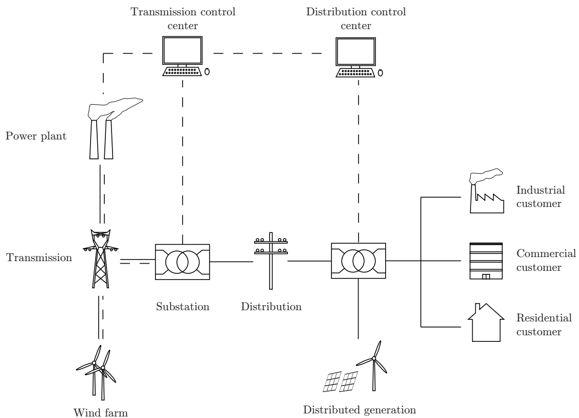
Figure 1.3: Architecture of current power systems, based on [3]. Plain lines indicate electrical infrastructures and dashed line communication channels.
