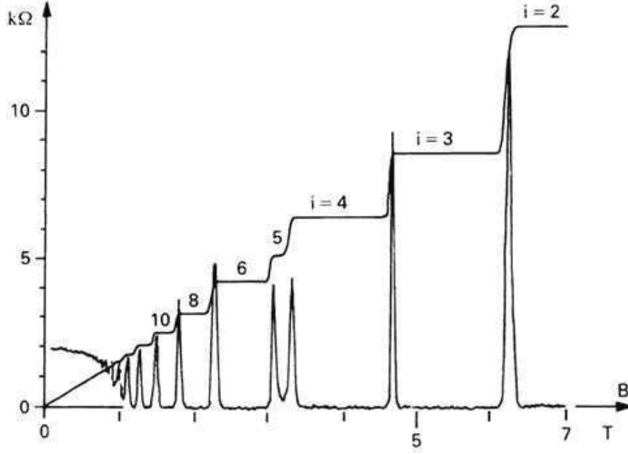
Figure 1.3: Plateaus for the Hall resistance and peaks of the Ohmic resistance in the integer quantum Hall effect. Neighboring values of i are separated by a quantum critical point, whose properties are described by a c = 0 2D (L)CFT. (figure taken from http://www.nobelprize.org/nobel_prizes/physics/laureates/1998/press.html ).
