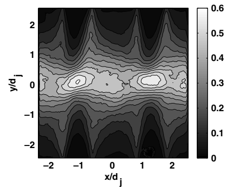
Fig. 5. Distribution of the normalized total kinetic energy \langle u_i u_i \rangle / V_{inj}^2 . Filled contour plot in increments of 0.1.
