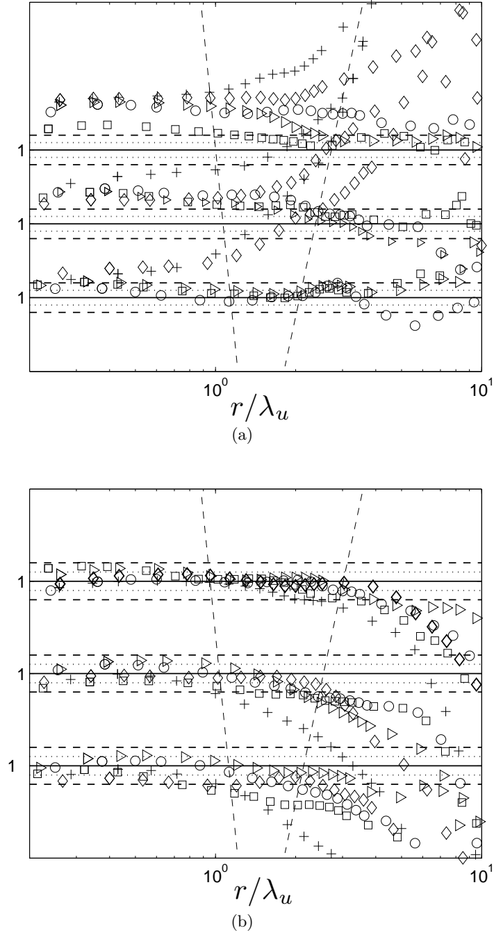
FIGURE 6. (a), (b) Ratio between measured and calculated third-order structure functions. Increasing Reynolds number from bottom to top. (a) \overline{\Delta u(\Delta v)^2} / \overline{\Delta u(\Delta v)^2}|_{iso} . (b) \overline{\Delta u(\Delta w)^2} / \overline{\Delta u(\Delta w)^2}|_{iso} . \circ CC, \square SqC, \diamond ScC, \triangleright P, + SS. — represents the isotropic ratio of 1, \cdots\cdots and - - - represent a departure of 10 and 20% respectively. The inclined vertical broken lines delineate approximately the extent of the restricted scaling range.
