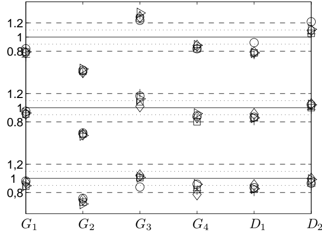
FIGURE 3. Velocity derivatives ratios G_1 , G_2 , G_3 , G_4 , D_1 , D_2 . \circ CC, \square SqC, \diamond ScC, \triangleright P, + SS. Increasing Reynolds number from bottom to top. — represents the isotropic ratio of 1, \cdots\cdots and - - - represent a departure of 10 and 20% respectively.
