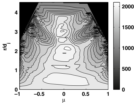
Fig. 8. Distribution of term \langle \epsilon \rangle + \langle \epsilon \rangle^+ in r, \mu coordinates.
