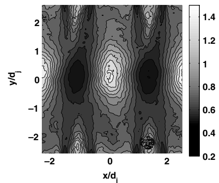
Fig. 4. Ratio \langle u^2 \rangle^{1/2} / \langle v^2 \rangle^{1/2} in the jet-axis plane.
