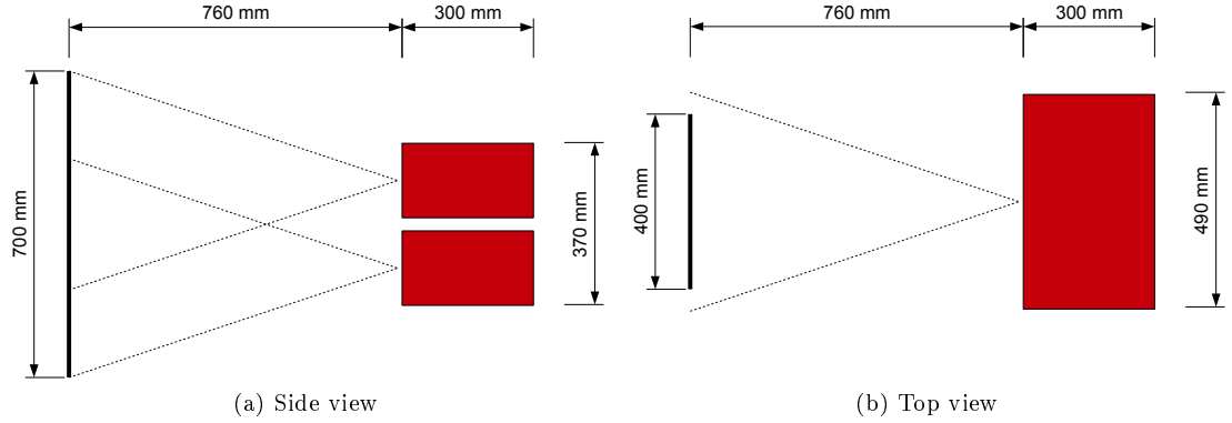
Figure 3.9: Top and bottom position of the Gom Atos III acquiring an area of 400 mm \times 700 mm.
