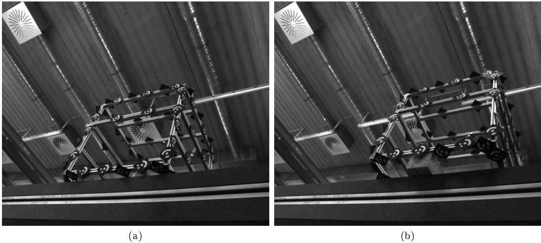
Figure 4.9: Target frame on the marble table seen from a bottom tracking camera. (a) representative of the badly tracked positions M1, M2 and M5. (b) representative of better tracked positions M3 and M4.
