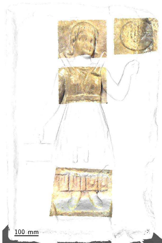
Figure 5.21: 3D – multispectral registration of the bas-relief data.
