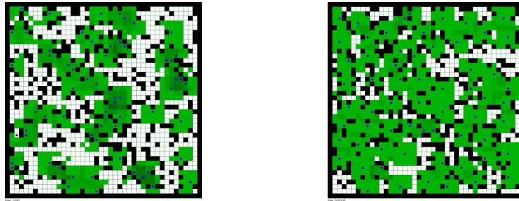
FIGURE 4.2 – Algorithme
