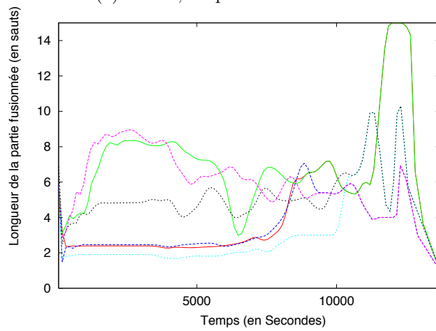
(b) \delta = 20 , Paquets de 400 octets.
