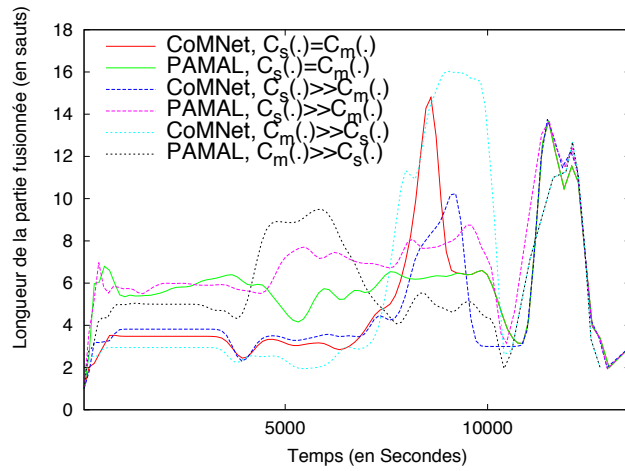
(a) \delta = 15 , Paquets de 400 octets.
