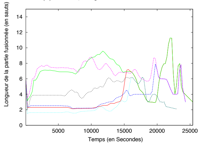
(b) \delta = 20 , Paquets de 200 octets.
