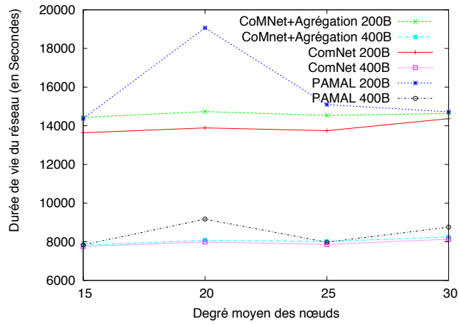
(a) C_{radio} = C_{mvt}
