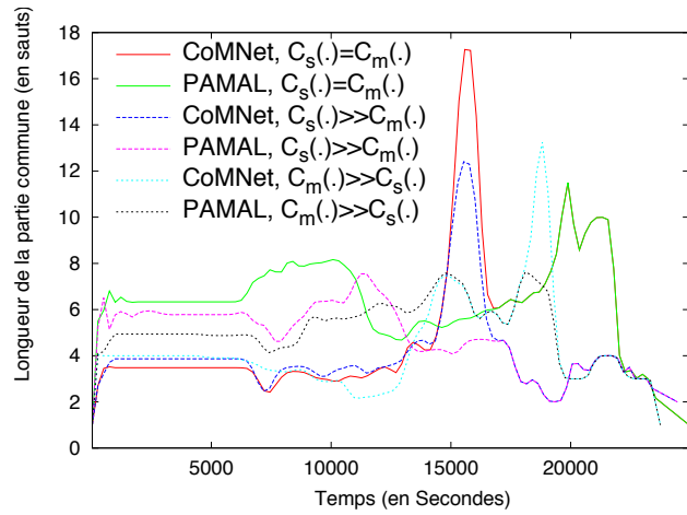
(a) \delta = 15 , Paquets de 200 octets.
