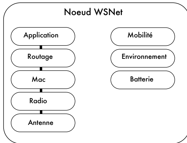
FIGURE 3.5 – Architecture WSNet
