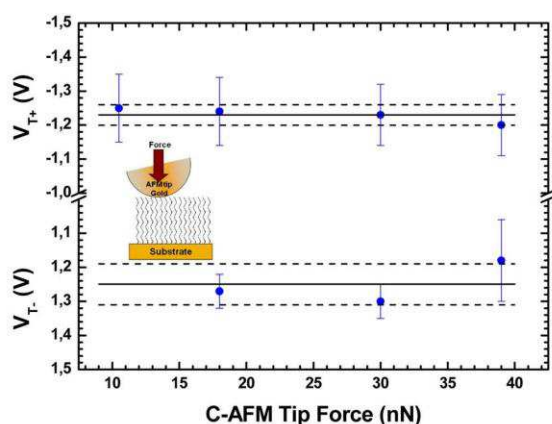
Figure 4. V_{T+} and V_{T-} determined from five I - V curves for the \text{Au-Si-C}_n\text{H}_{2n+1} ( n = 12 ) junction as a function of the loading force on the AFM tip. The solid lines correspond to the average value for V_T , and the dashed lines show the standard deviation.
