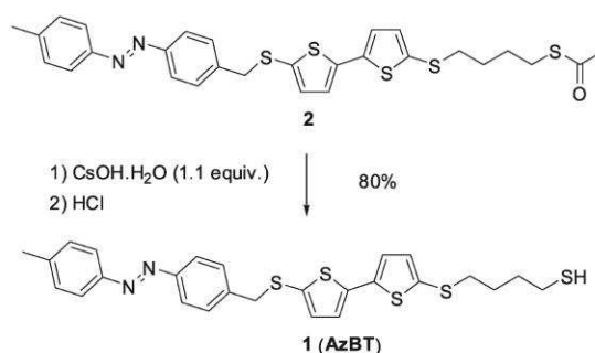
Scheme 1. Chemical structures of the molecules.
