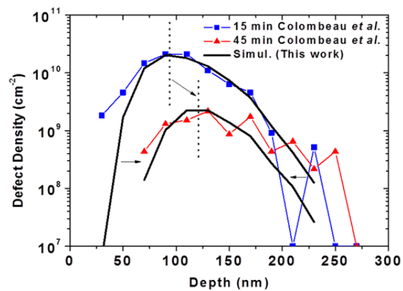
Figure 32 – Time evolution of the mean depth of the defects formed by 40 keV, 6 \times 10^{13} \text{ cm}^{-2} Si implant annealed at 740 °C. The mean depth increases with time. (From Ref. 26)
