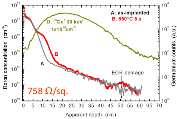
Figure 5 – SIMS profiles of as-implanted (labelled “A”) and SPEG processed (650°C 5 s, labelled “B”) boron distribution (0.5 keV, 1 \times 10^{15} \text{ cm}^{-2} ). Also shown is the Ge 3+ 30 keV 1 \times 10^{15} \text{ cm}^{-2} as-implanted profile.
