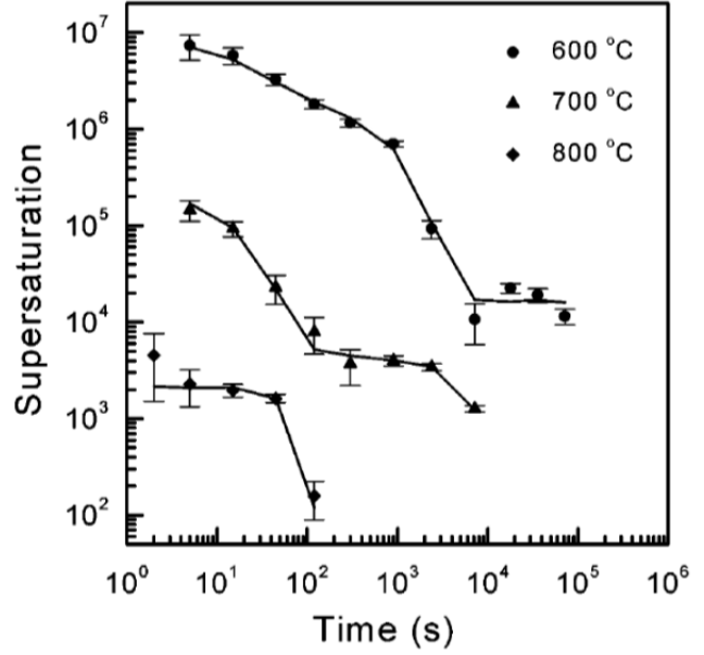
Figure 6 – Interstitial supersaturation, S , as a function of annealing temperature and time. Symbols: experimental values. Lines: fits based on Ostwald ripening model (From Ref. 19)
