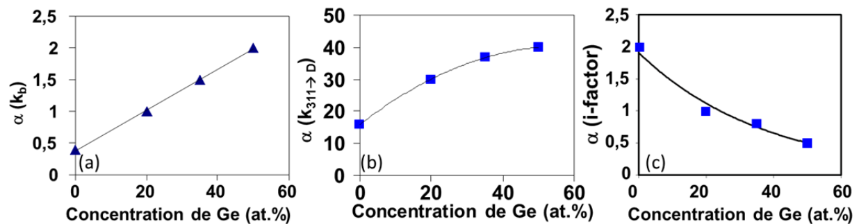
Figure 23 – Ge-content dependence of the correction multiplying factor applied to the default parameters of the “moment-based” defect model: (a) {311}s emission rate, (b) {311} \rightarrow DLs transformation rate and (c) i-factor .
