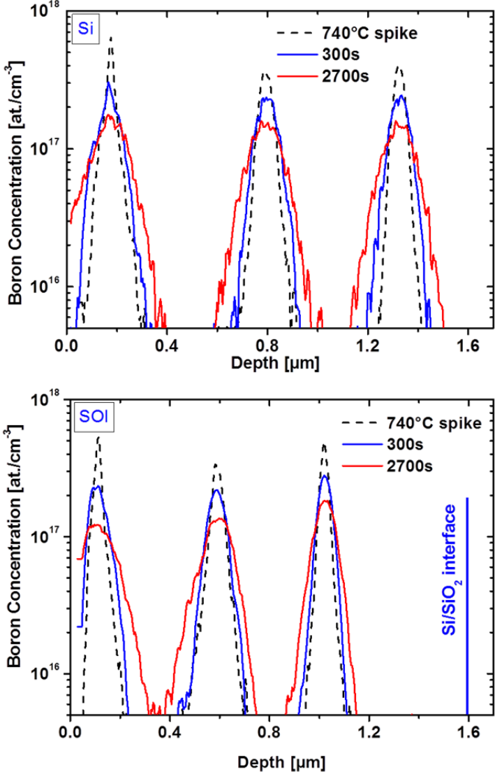
Figure 14 – Boron depth distribution profiles in (a) Si and (b) SOI structures measured by SIMS following a 40 keV Si + implant to a dose of 6x10 13 cm -2 and annealing at 740 °C for various time intervals.
