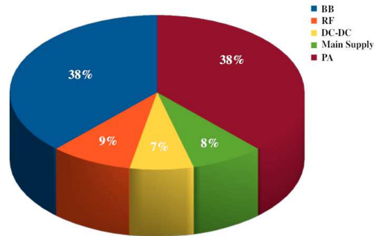
(b) Station de base micro [ABG10]. PA : Power Amplifier, BB : Baseband interface, RF : Radio Frequency transceiver.
