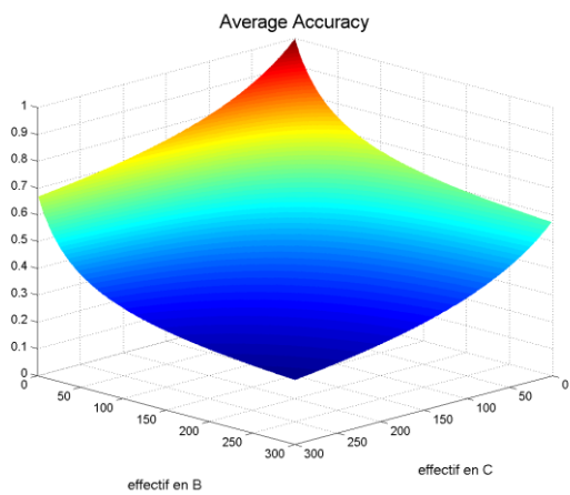
figure II.9 : Simulation de l'indice AA
