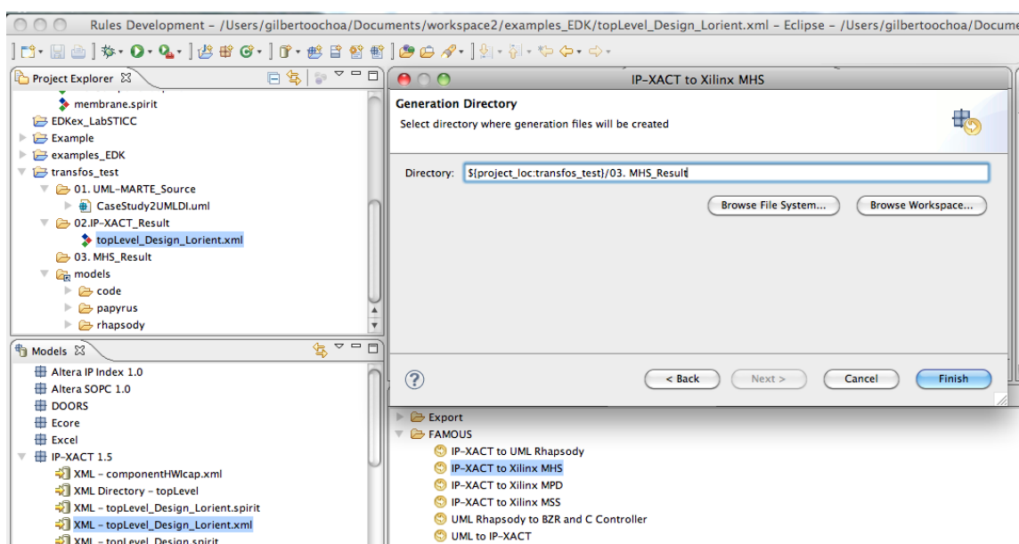
Figure 6.17: Example of the compilation chain in Sodi MDWorkbench
