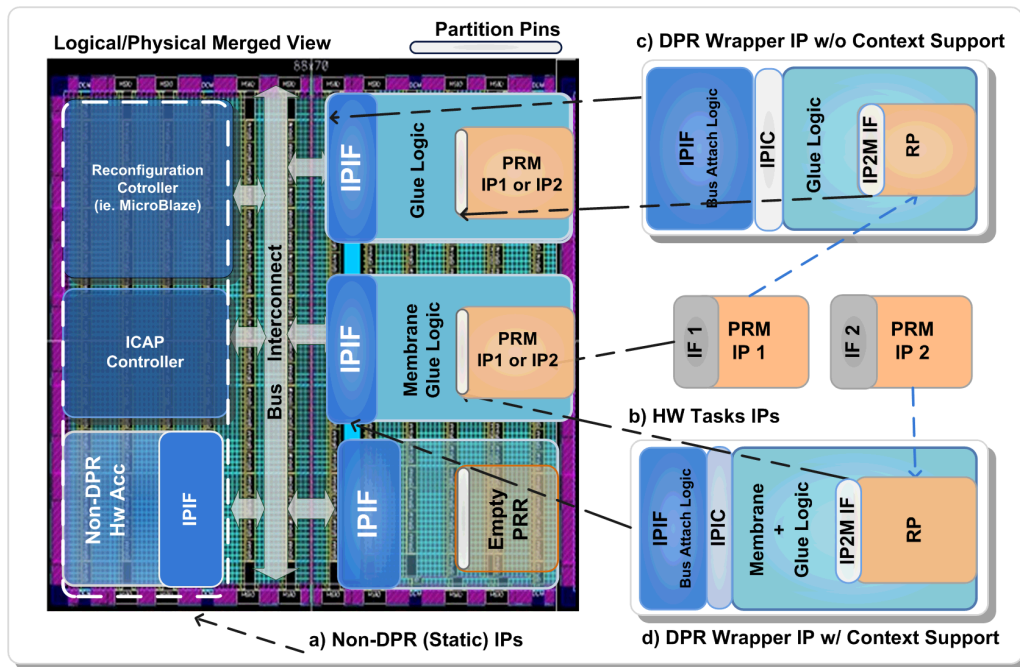
Figure 4.8: Classification of different IPs in the FAMOUS approach
