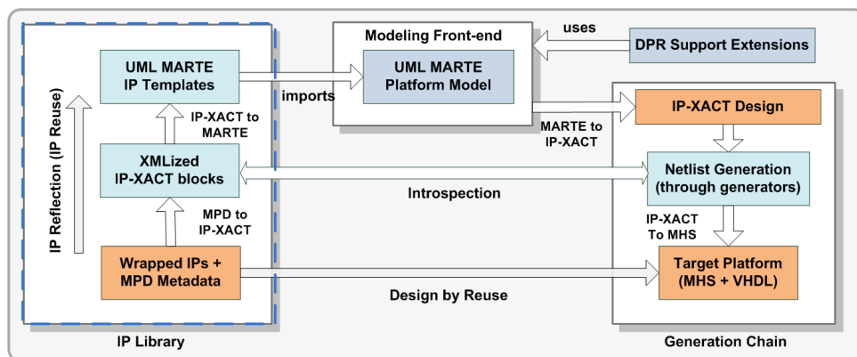
Figure 5.1: Metadata Reflection for IP reuse phase of the FAMOUS Methodology
