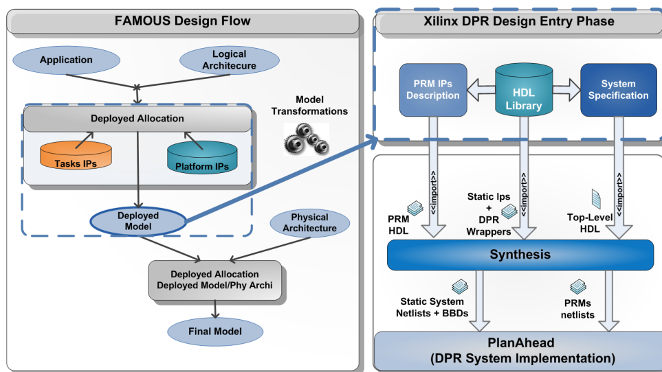
Figure 1.15: The proposed MDE approach (a) and its interactions with the PR design flow (b)
