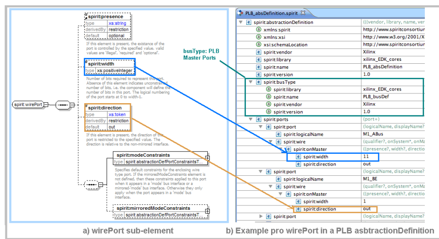
Figure 5.10: Example of a wirePort element (a) and its use in an asbtractionDefinition (b)
