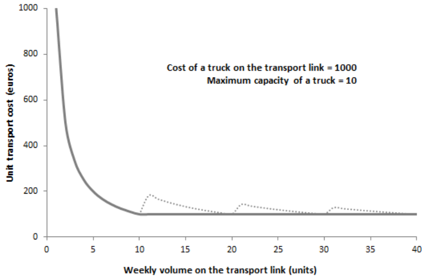
Fig. 1.12 Unit cost as a function of the weekly transported volume on a given transport link.
