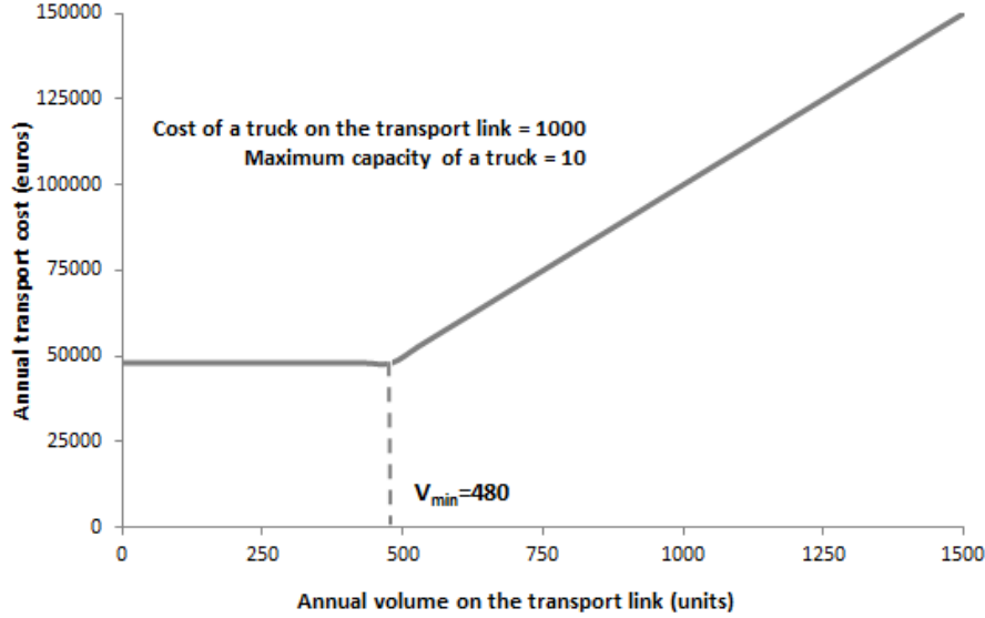
Fig. 4.3 Example of the annual transport cost as a function of the annual transported volume on a given link where the cost of a truck is set to 1000 and its capacity to 10.
