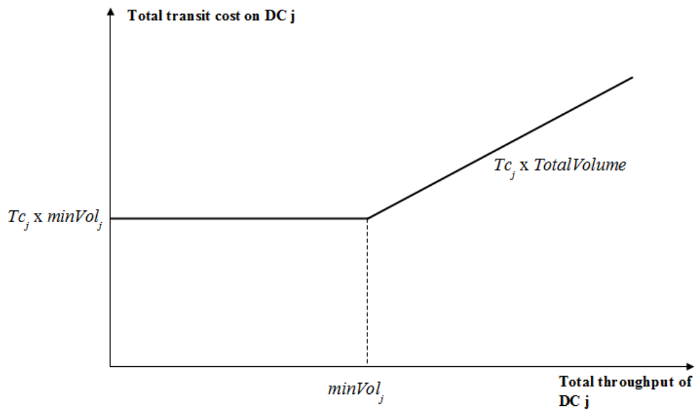
Fig. 5.6 Total transit cost as a function of throughput for a given DC j when using unit transit cost as penalty for violating minimum volume constraints on DC j .
