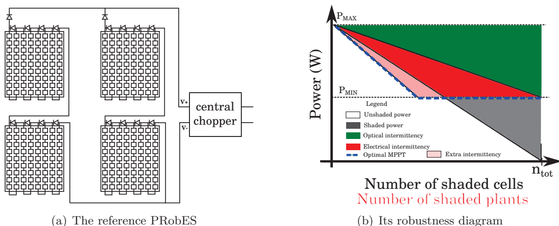
Figure 2.42: The reference PRobES and its robustness diagram
