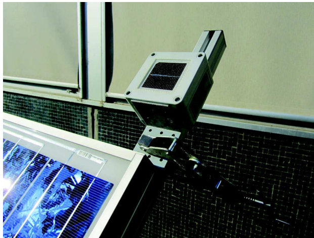
Figure B.4: The reference cell
