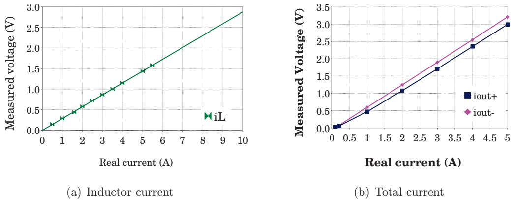
Figure B.13: Ratings for the different currents
