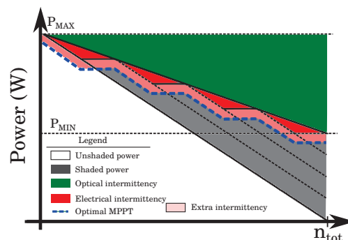
(b) Module series PRobES robustness diagram
