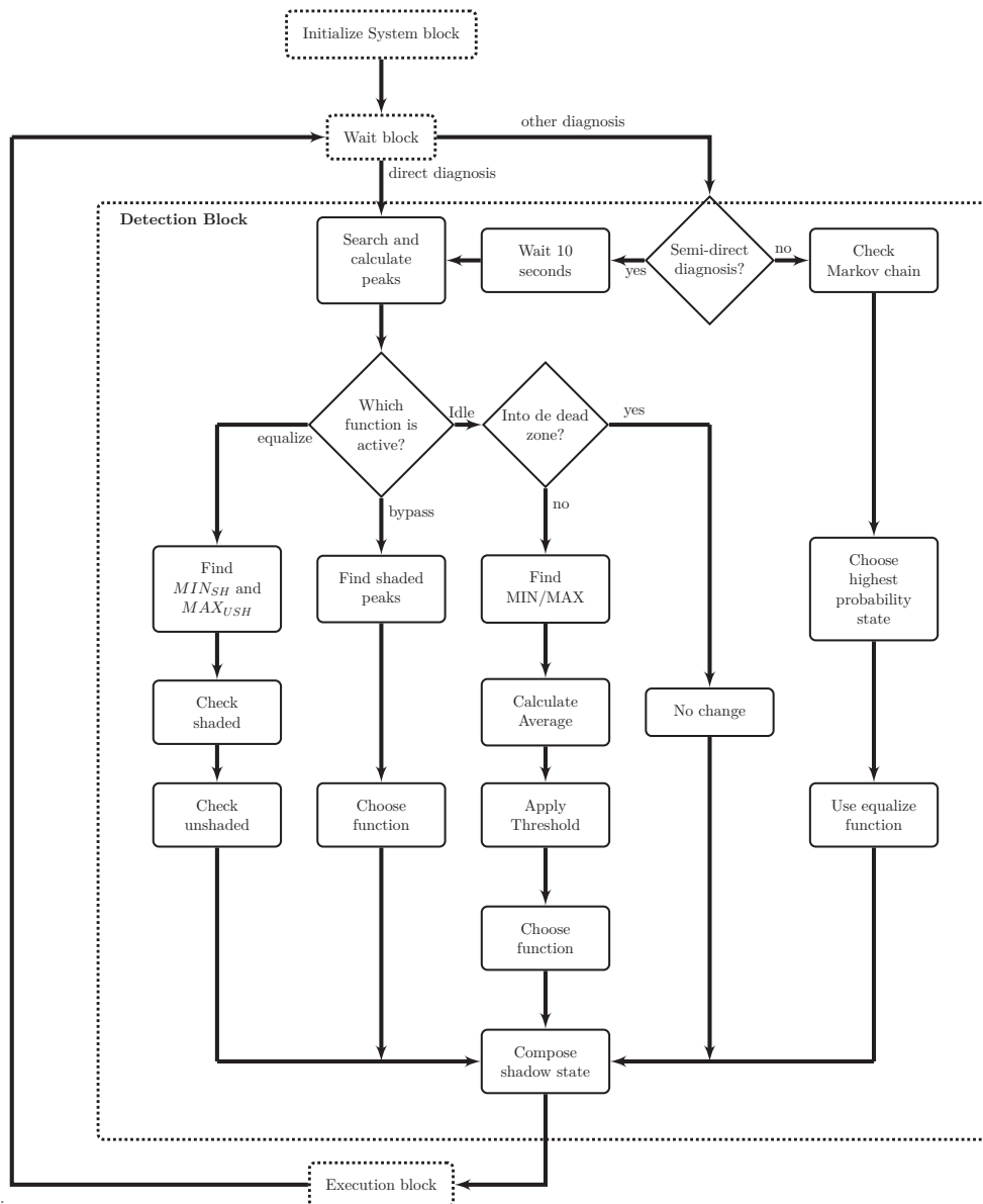
Figure 6.9: Detection algorithm
