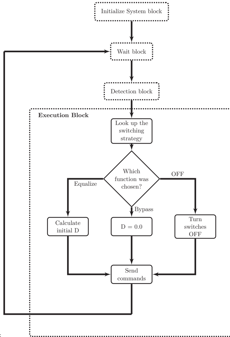
Figure 6.12: Execution algorithm
