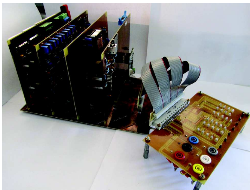
Figure B.17: All cards connected to the interconnection card
