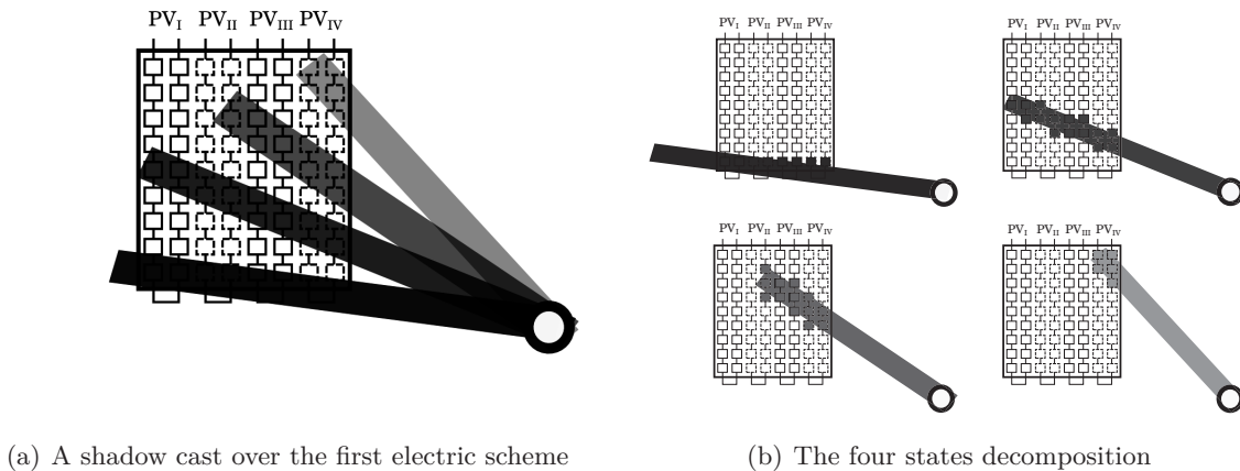
Figure 2.23: Impact of a shadow over the first electric scheme
