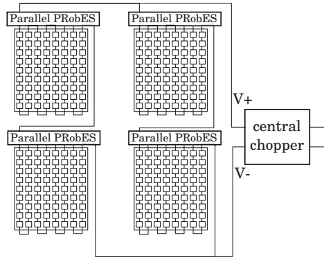
(a) A PV plant equipped with parallel PRobES
