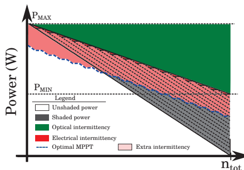
(b) Micro-converters series PRobES robustness diagram
