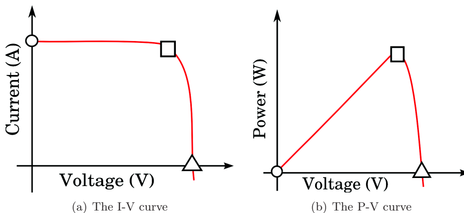
Figure 2.3: The characteristic PV curves
