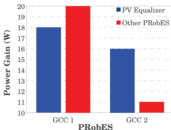
Figure 7.2: Absolute power gain comparison between the PV Equalizer and the GCC
