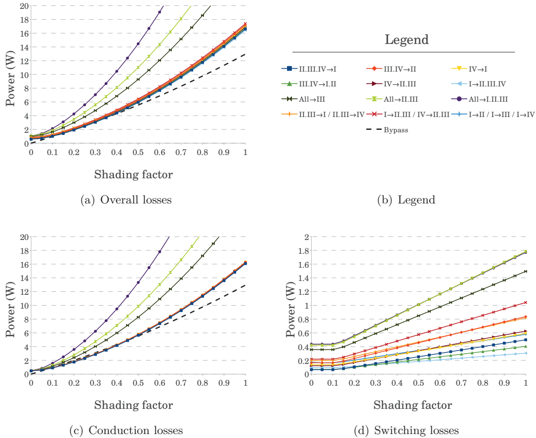
Figure 3.21: Equalizer losses
