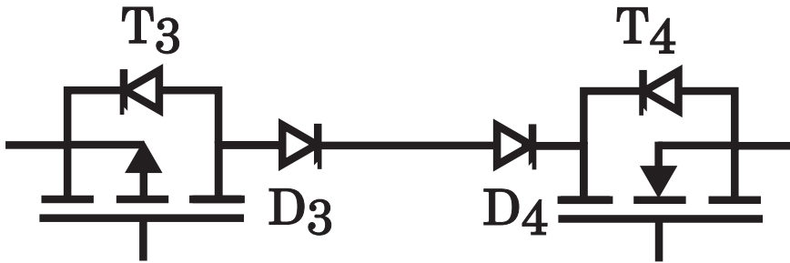
Figure B.15: The real switching leg
