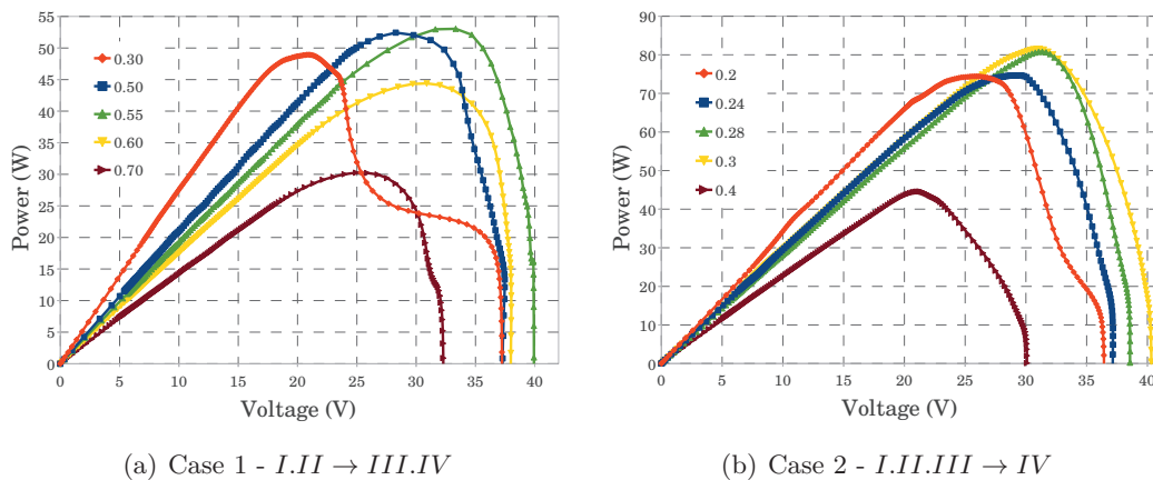
Figure 4.12: Experimental P-V curves for the BSS
