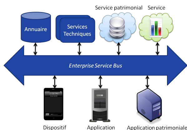
FIGURE 3.8 – Architecture ESB.
