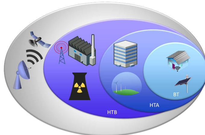
FIGURE 1.1 – Infrastructure générale.
