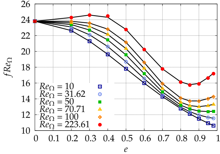
Figure 3.6 – Comparison of Fanning friction factor with numerical values of Escudier et al. (2000), for \eta = 0.5 . The values of Re_{\Omega} correspond to Taylor numbers Ta = Re_{\Omega}^2 \delta = 1000, 2500, 5000, 10000, 50000 . Lines: present results; symbols: Escudier et al. (2000).
