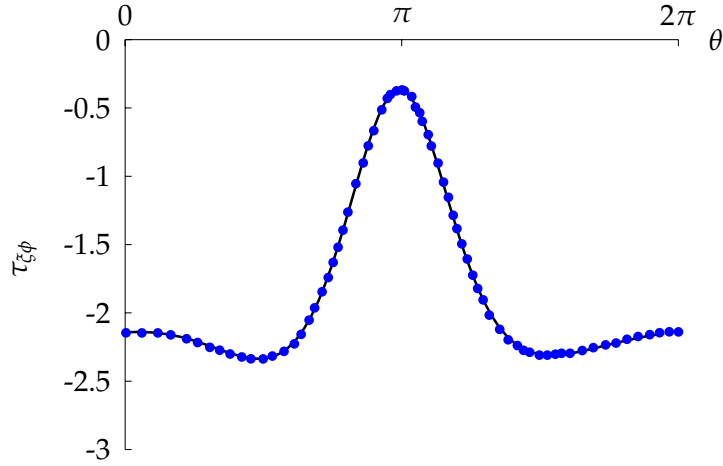
Figure 3.7 – Shear stress \tau_{\xi\phi} acting on the inner cylinder non-dimensionalized by \mu a \Omega / d , for \delta = 0.205 , e = 0.5 , Re_{\Omega} = 155 . Comparison with figure 8 in Oikawa et al. (1989a). Lines: present results; symbols: Oikawa et al. (1989a).
