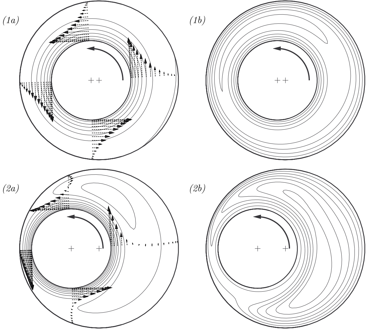
Figure 5.3 – Basic flows for Re_{\Omega} = 500 : (1) weak eccentricity e = 0.2 , (2) high eccentricity e = 0.7 . (a) Contours of equispaced in-plane streamfunction with superimposed \mathbf{U}_{\perp} profiles at \theta = 0, \pi/2, \pi, 3\pi/2 (polar angle with respect to the inner cylinder). (b) Equispaced contours of W .
