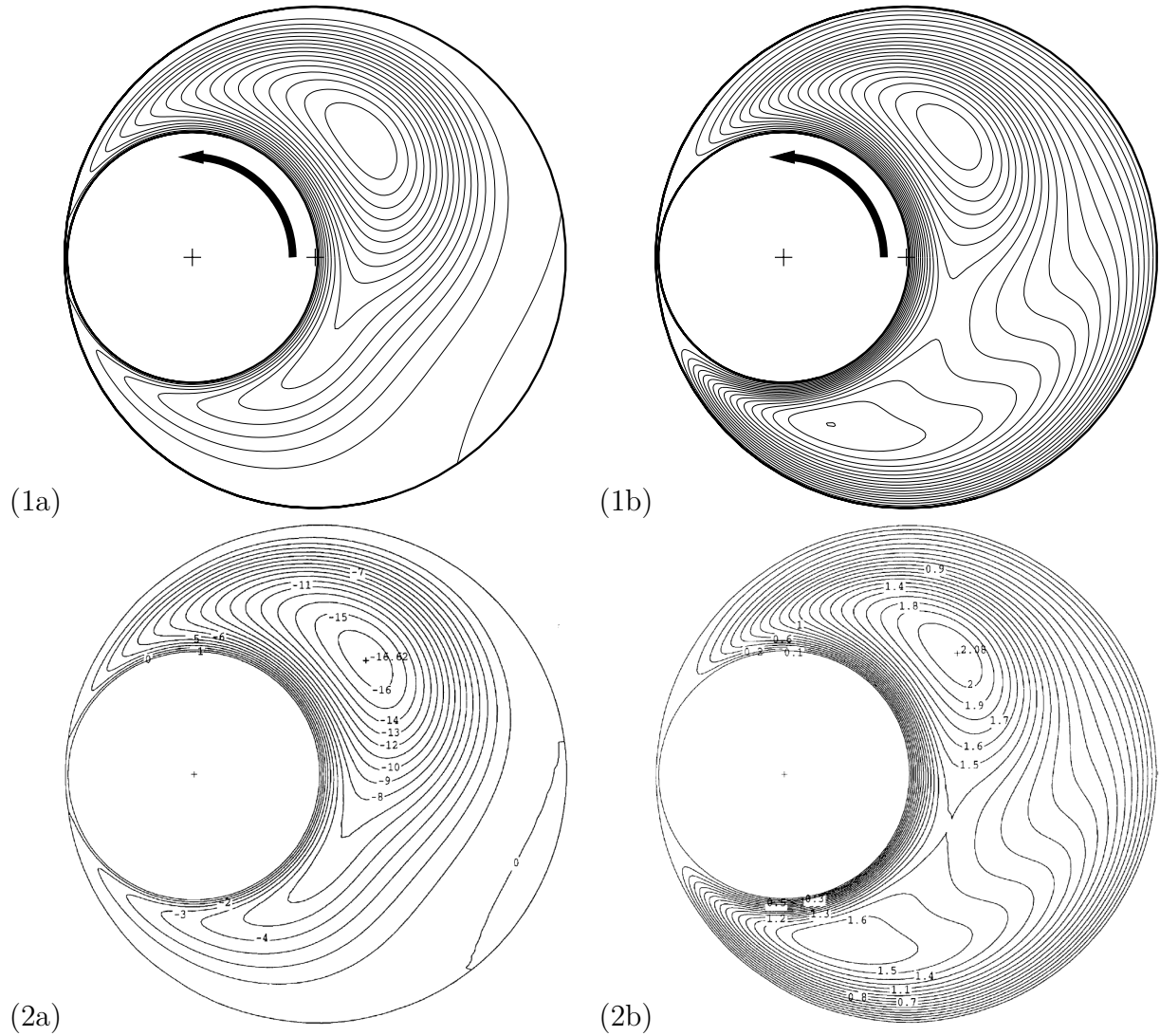
Figure 3.10 – Streamlines (a) and axial flow isocontours (b) for \eta = 0.5 , e = 0.98 and Re_\Omega = 223.61 . Comparison of (1) present calculations using (M + 1) \times N = 32 \times 257 ( K = 128 ) with (2) Escudier et al. (2000). The calculation recovers the secondary recirculation region in the wide gap and the two distorted maxima in axial velocity. The numerical values of the isolines match those of Escudier et al. (2000).
