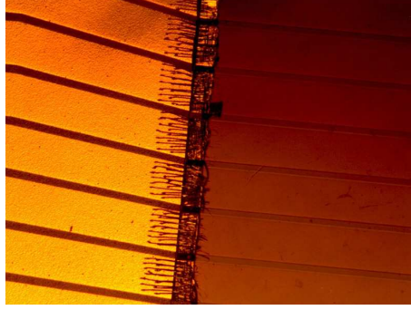
Figure A.3.: Electric connection between the base chip (left) and the science chip (right) with 14 bonding wires per chip wire.
