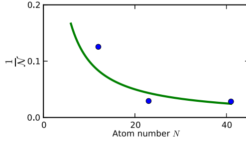
Figure 4.15.: Remnant fidelity \frac{1}{N} at \tau \rightarrow \infty for the W states with three different atom numbers. The values are obtained from the fit to the decoherence measurement shown in figure 4.14. The green curve shows the expected 1/N dependence.
