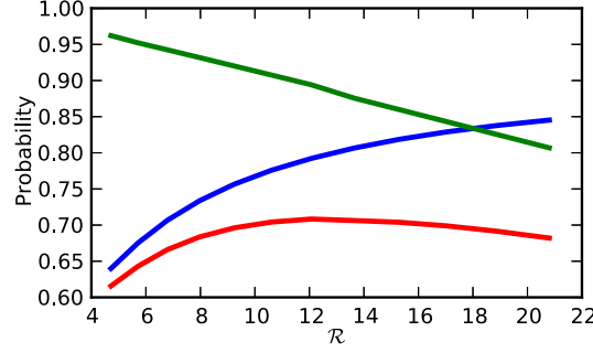
Figure 6.4.: The Fidelity \rho_{11} (blue curve) and the probability for no scattering events ( 1 - p_{sc} ) during the W state preparation (green curve) in dependence of \mathcal{R} for N=10 atoms. The red curve shows the product \rho_{11} \cdot (1 - p_{sc}) . It is maximal for \mathcal{R} = 12.1 .
