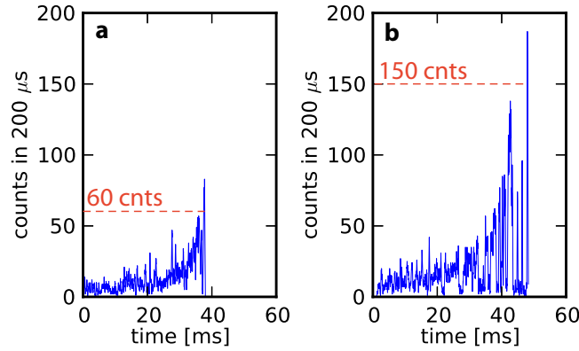
Figure 3.6.: a) Typical transmission signal during the atom number preparation. When the count rate exceeds 60 counts in 200\text{ }\mu\text{s} , the light is switched off and we end up with a well defined atom number in the cavity. b) Transmission trace for a threshold T_{\text{prep}} = T_{\text{max}}/2 . The lifetime for atoms in F = 2 is increased when the cavity is close to resonance (in this trace for times higher than 40\text{ ms} ). This leads to longer periods of low transmission and increases the uncertainty of the prepared atom number.
