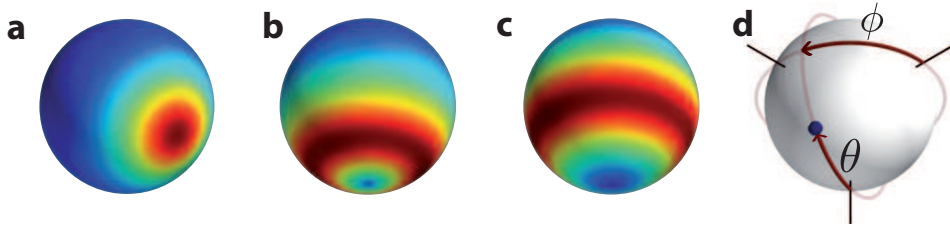
Figure 4.4.: Representation of the Q function on the multiparticle Bloch sphere for different states. a) CSS |\theta = 0.8, \phi = 0\rangle containing 20 atoms. b) Dicke state |n = 2_{N=20}\rangle . c) Dicke state |n = 5_{N=20}\rangle . d) Coordinate system used in a), b) and c). This representation is also used in all the following drawings of a multiparticle Bloch sphere.
