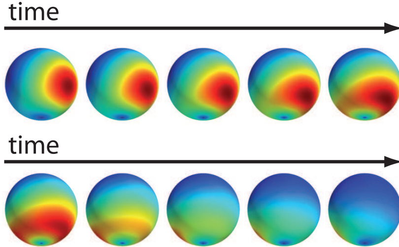
Figure 6.2.: The evolution of the state from figure 6.1 (red curve) on the Bloch sphere. The south pole is never populated, because the constant measurement prevents the occupation of the state |0_N\rangle . When the (initially coherent) state approaches the south pole, it splits and encircles it. At t = \pi/\Omega_Z (first image, second row), the overlap with the W state is maximal.
