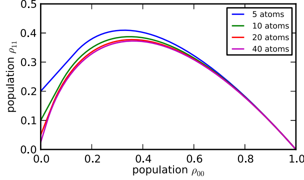
Figure 5.8.: The entanglement criterion from figure 5.7 extended to mixed states. The populations \rho_{00} and \rho_{11} of a separable state with a certain atom number - mixed or pure - can only lie in the area below the corresponding threshold. If a state has populations above the threshold, it must be entangled.
