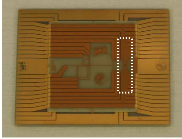
Figure 2.11.: A photo of the atom chip used in the experiment. It consists of two chips made of Aluminium Nitride that are glued together. The wires on the chip substrates are made of gold and are grown on the substrate by galvanic deposition. The two chips are electrically connected by bond wires. In this image, the fibre cavity is not yet glued to the chip. Its later position is indicated by the dotted line.
