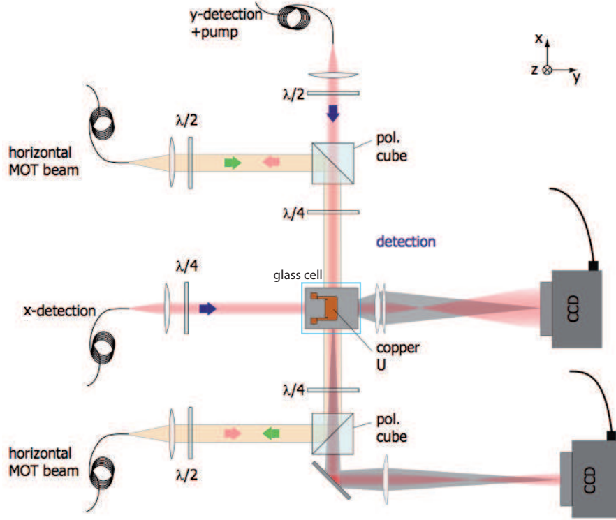
Figure 2.7.: Schematic of the optical setup surrounding the glass cell (top view). Two of the four MOT beams are shown. The other two beams hit the chip under an angle of 45^\circ and are reflected by the chip surface to create a mirror-MOT. The two detection beams allow to make absorption images of the atomic cloud in the MOT region (y-detection) and in the cavity region (x-detection). Adapted from [55].
