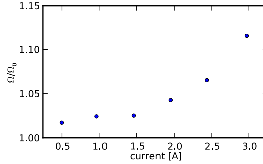
Figure A.7.: Relative resistance of the MIWG wire in dependence of the current after 10s.
