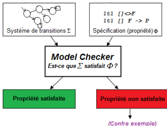
Figure 3.1 Principe du model-checking.
