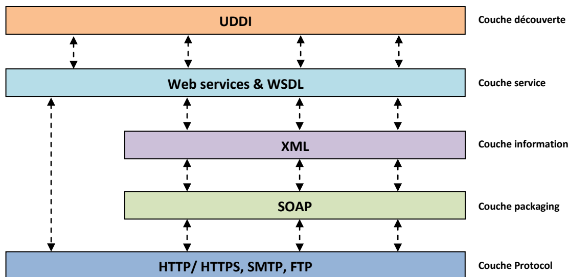
Figure 1.6 Pile de protocoles de services web
