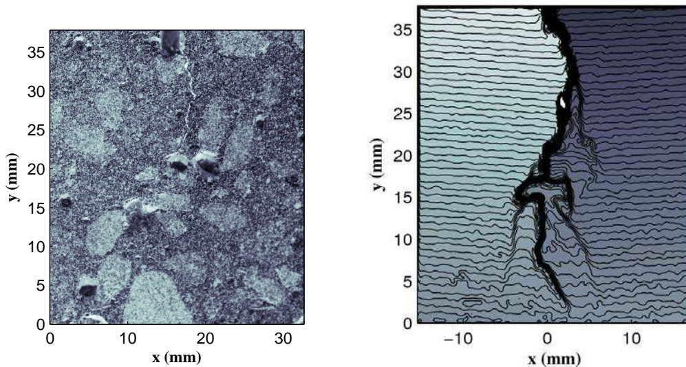
Figure 4.3: (a) Picture of a specimen surface after mechanical loading, (b) surface displacement mapping of a concrete sample from Digital Image Correlation ( 5 \mu\text{m}/\text{line} )
