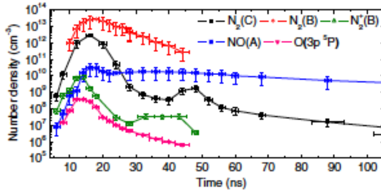
Figure 2.24: Number density of excited species measured at mid gap for a typical NRP Glow discharge. T_g = 1000 K, d = 5 mm, V_p = 6.7 kV, PRF = 30 kHz, and v = 2 m.s ^{-1} . Figure taken from [36].
