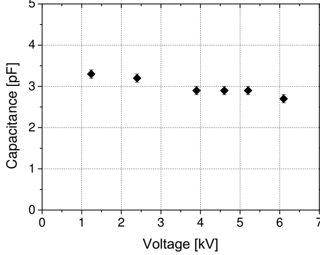
Figure C.5: Electrode capacitance C as a function of the applied voltage for different "no discharge" state at room temperature.
