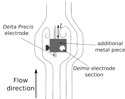
Figure 6.2: Schematic diagram presenting the nature of the flow before and after the obstacle. The carrying Delmo electrode direction is orthogonal to the figure plane.
