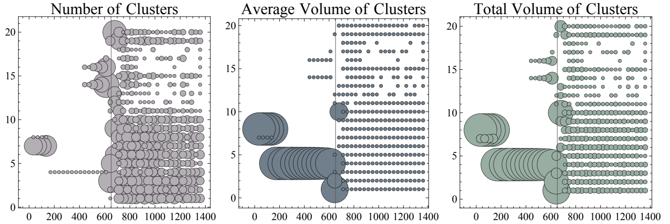
Fig. 3.33: \text{PZ}_{60}\text{T}_{40} : Temperature evolution of the number of clusters ( N_{Cl} ), their average volume ( V_{Cl}^{av} ) and their total volume ( V_{Cl}^{tot} ) per face. The y axis refers to the face label, the x axis denotes temperature. Let's first put our attention on the high-temperature region. (i) High temperatures are characterized by small values of N_{Cl} , V_{Cl}^{av} and V_{Cl}^{tot} for all faces. Thus spatial correlations are very weak, and all directions are equivalent. This is merely indicative of full disorder. (ii) While approaching T_C (indicated by a vertical line) from above, one observes signatures of critical fluctuations, such as emergence of preferred orientations (some directions are no longer represented while large spatial clusters corresponding to certain equivalent rhombohedral orientations appear) and scale invariance (indicated by the fact that differently populated directions acquire equal number of clusters). (iii) Below T_C , up to \sim 440\text{K} , one observes the condensation of only several clusters oriented in [1, -1, 1] and [1, -1, -1] directions (faces 4, 14 and 16). Whereas the single cluster corresponding to [1, -1, 1] (major phase) direction stands out in terms of large volume, the clusters with [1, -1, -1] (minor phase) orientation are numerous and, in contrast, relatively much smaller in volume. This latter observation shows that below T_C the percolation of [1, -1, 1] clusters has been achieved, however the volume corresponding to the major phase is not simply connected. This situation is not persistent since a further decrease of the temperature drives this minor phase to gradually shrink, ultimately disappearing at 440\text{K} . (iv) At temperatures below \sim 440\text{K} the ground state is achieved. It is important to mention that what could appear as a switching of direction is, in fact, only an artifact of Metropolis Monte-Carlo method.
