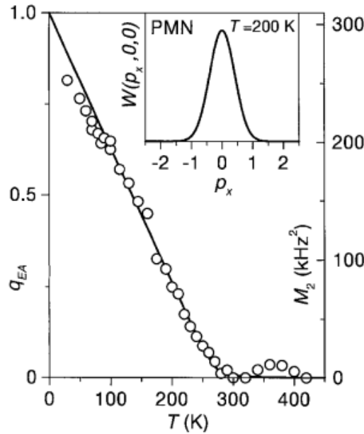
Fig. 1.26: Temperature dependence of the Edwards-Anderson order parameter q_{EA} of the reorientable part of the inhomogeneous frequency distribution in PMN ( q_{EA} \propto M_2 ). The inset shows the Gaussian shape of the probability distribution of local polarization. (After Blinc et al. [99])
