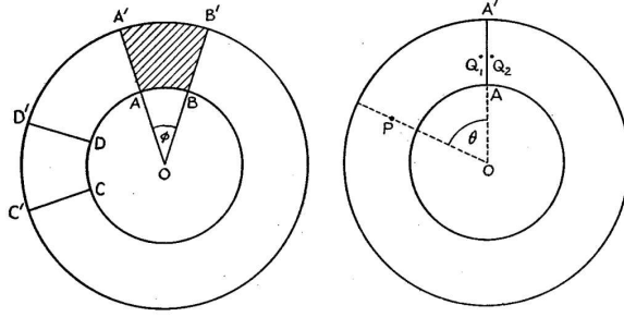
Fig. 2.15: Left Dislocation of a hollow ring. The ring is cut along the radial lines AA' and BB' , the wedge AA'B'B' is removed, and AA' is joined to BB' . The same dislocation could be made by cutting along CC' and DD' . Right The dislocated ring. The neighbouring points Q_1 and Q_2 lie on opposite sides of the cut (after Nabarro [211])
