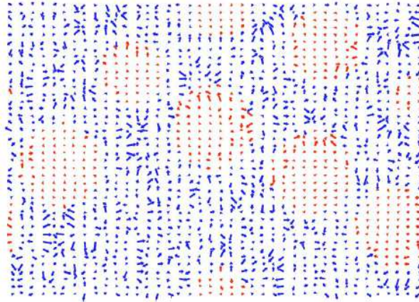
Fig. 1.20: Projection of the Pb-site local fields (in arbitrary units) on a (110) plane through the simulation box of \text{Pb}(\text{Sc}_{1/2}\text{Nb}_{1/2})\text{O}_3 . Chemically ordered regions have relatively small homogeneous fields whereas chemically disordered regions have larger, more varied disordered local fields. (After Burton et al. [146])
