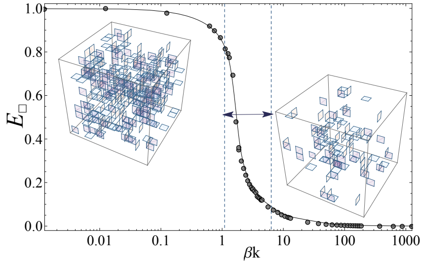
Fig. 2.29: The plaquette energy E_{\square} as a function of \beta k , with k the gauge coupling parameter and \beta the inverse temperature, on a 12^3 cubic lattice with cold start configuration ( i.e. all links are initially set to unit matrices). The temperature is kept fixed at high values in the course of this simulation. Right and left insets show snapshots of plaquettes \mathbf{U}_{\square} that deviate from unity for high and low values of \beta k , respectively.
