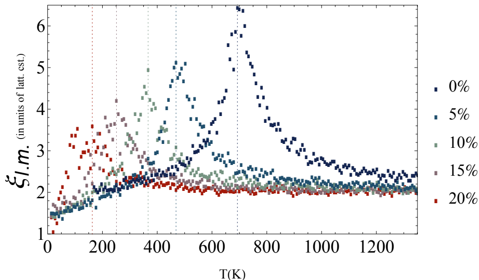
Fig. 3.17: Temperature evolution of the correlation length of the the local modes \xi_{l.m.} for \text{PZ}_{60}\text{T}_{40} , \text{PL}_5\text{Z}_{60}\text{T}_{40} , \text{PL}_{10}\text{Z}_{60}\text{T}_{40} , \text{PL}_{15}\text{Z}_{60}\text{T}_{40} and \text{PL}_{20}\text{Z}_{60}\text{T}_{40} systems. Dotted vertical lines refer to the temperatures at which the correlation lengths peak.
