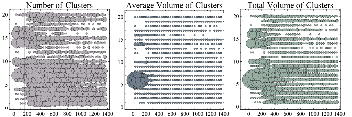
Fig. 3.36: PL_{15}Z_{60}T_{40} : Temperature evolution of the number of clusters ( N_{Cl} ), their average volume ( V_{Cl}^{av} ) and their total volume ( V_{Cl}^{tot} ) per face. The y axis refers to the face label, the x axis denotes temperature. (i) The high temperature range exhibits full-disorder characteristics. (ii) Above T_C , faces 6, 14 and 16 exhibit a monotonical increase of V_{Cl}^{tot} and of V_{Cl}^{av} . The fact that V_{Cl}^{av} also increases in the case of PL_{15}Z_{60}T_{40} is an indication of a more developed local order. (iii) Below T_C , large volumes of differently ordered regions make the ground state direction mixed between different directions, mainly composed of the directions [1, -1, -1] (faces 6, 7, 14 and 16) and [-1, -1, -1] (faces 10, 20), making the average symmetry monoclinic on the verge of being triclinic (section 3.1.5).
