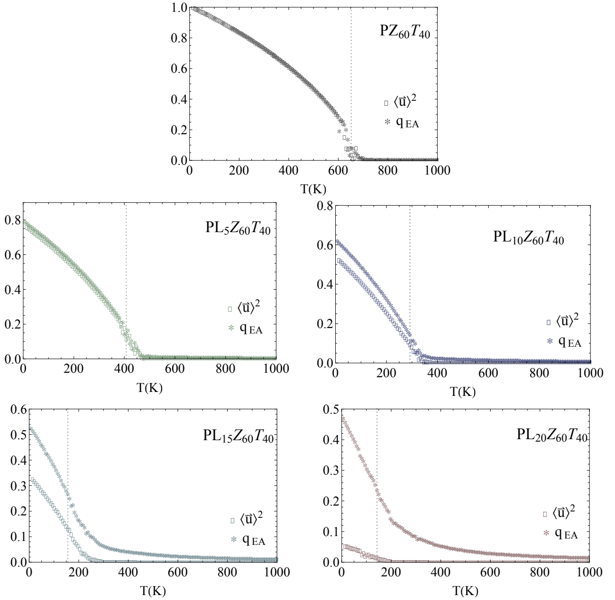
Fig. 3.26: Temperature evolutions of the Edwards-Anderson parameter q_{EA} and squared polarization \langle \bar{u} \rangle^2 , for PZT, PL 5 ZT, PL 10 ZT, PL 15 ZT and PL 20 ZT systems. Dotted vertical lines correspond to T_C ( i.e. , the temperature at which the specific heat peaks).
