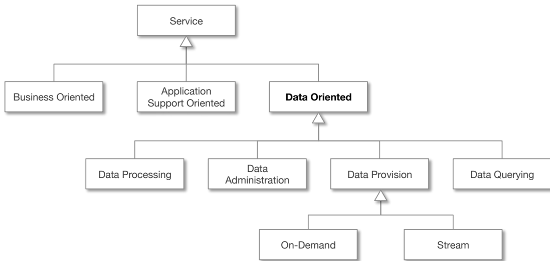
Figure 2.1 Service classification (UML class diagram)
