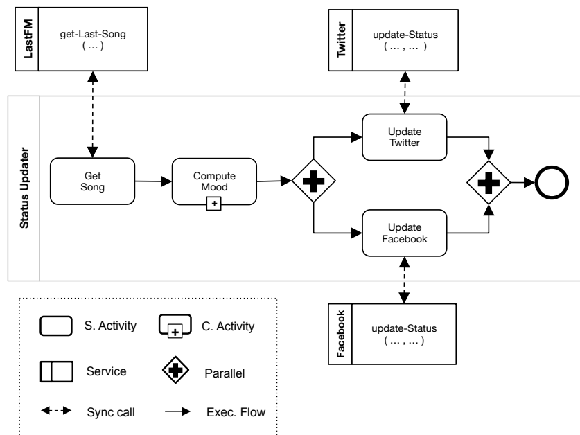
Figure 2.11 Workflow example
