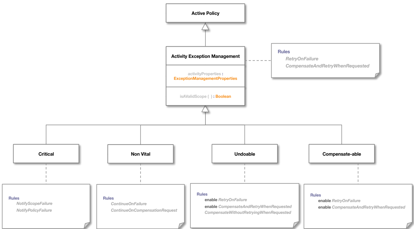
Figure 5.5 Exception Management Active Policy type (UML class diagram)
