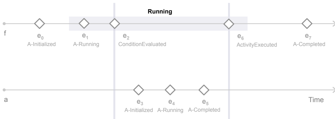
Figure 4.13 Event trace produced by the normal execution of an IF activity instance
