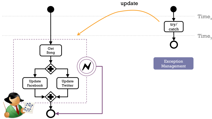
Figure 4.38 Exception handling: example of control flow and memory intrusive FR and NFR workflows
