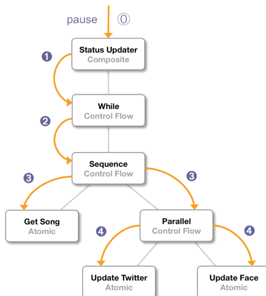
Figure 4.2 Behavior of a composite activity when "paused"
