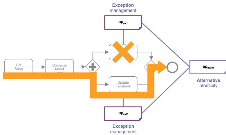
Figure 5.6 ForwardRecovery principle
