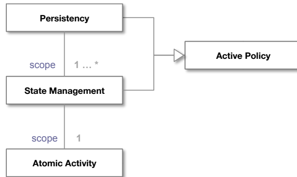
Figure 5.8 Persistence and State Management types relationships (UML class diagram)
