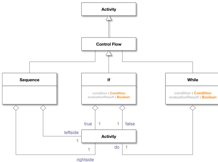
Figure 3.14 Control Flow activity type UML class diagram
