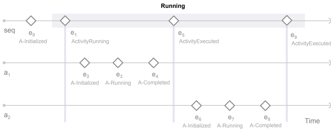
Figure 4.10 Event trace of Sequence activity normal execution
