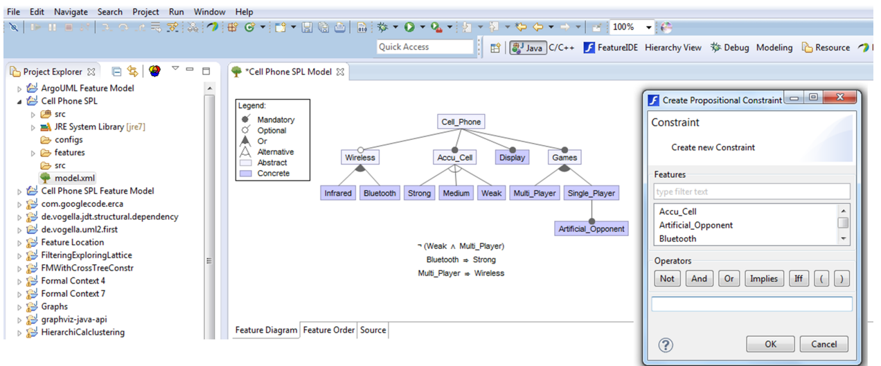
Figure A.9 : The graphical feature model editor of FeatureIDE.
