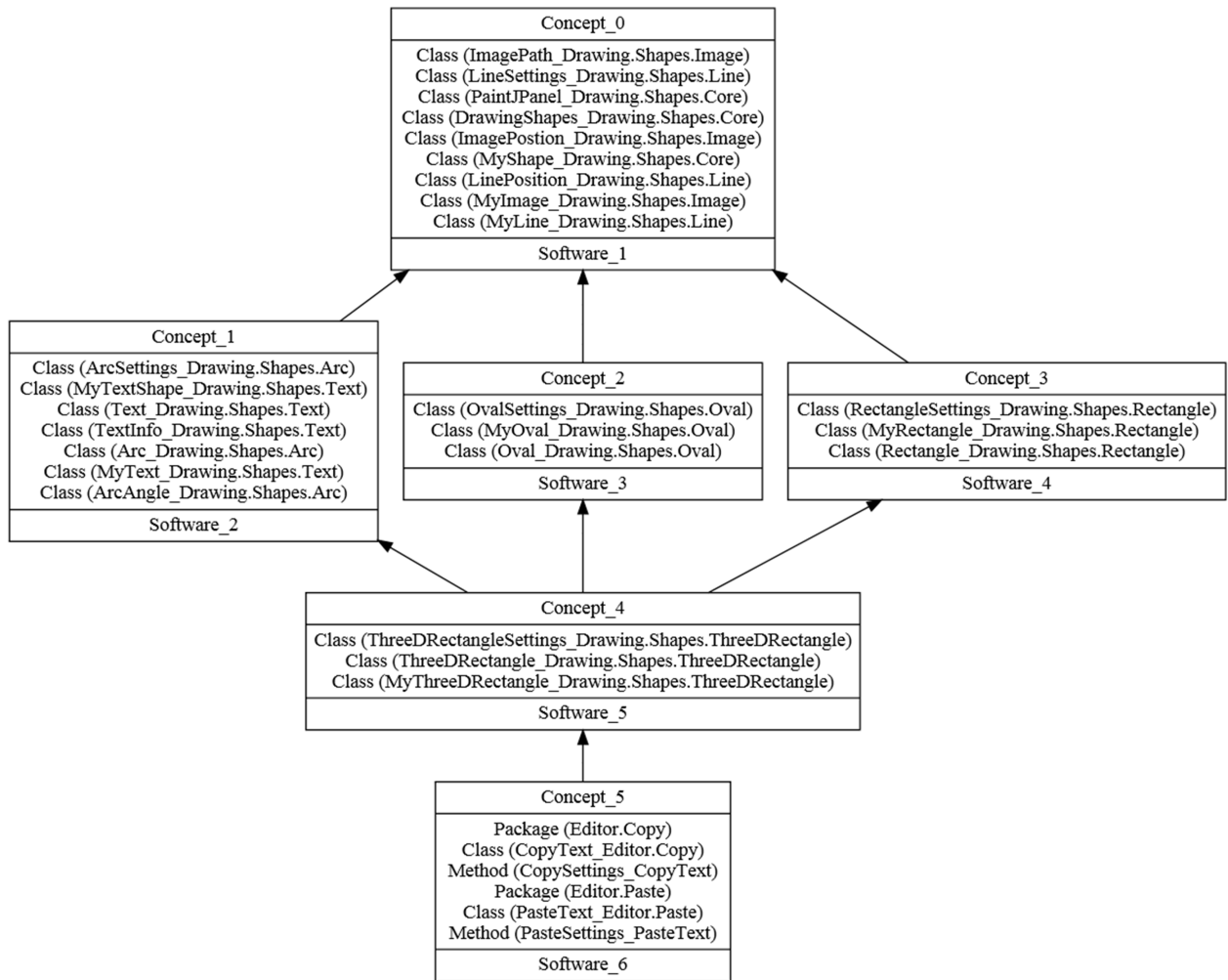
Figure 4.6 : The AOC-poset for the formal context of Table 4.2.
