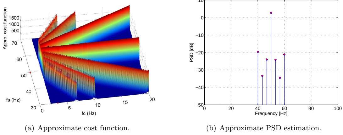
Figure 2.6: Approximate cost function \mathcal{J}_a(\Omega) and signal PSD ( f_s = 50\text{Hz} , f_c = 10\text{Hz} and L = 2 ) for a wrong value of model order.
