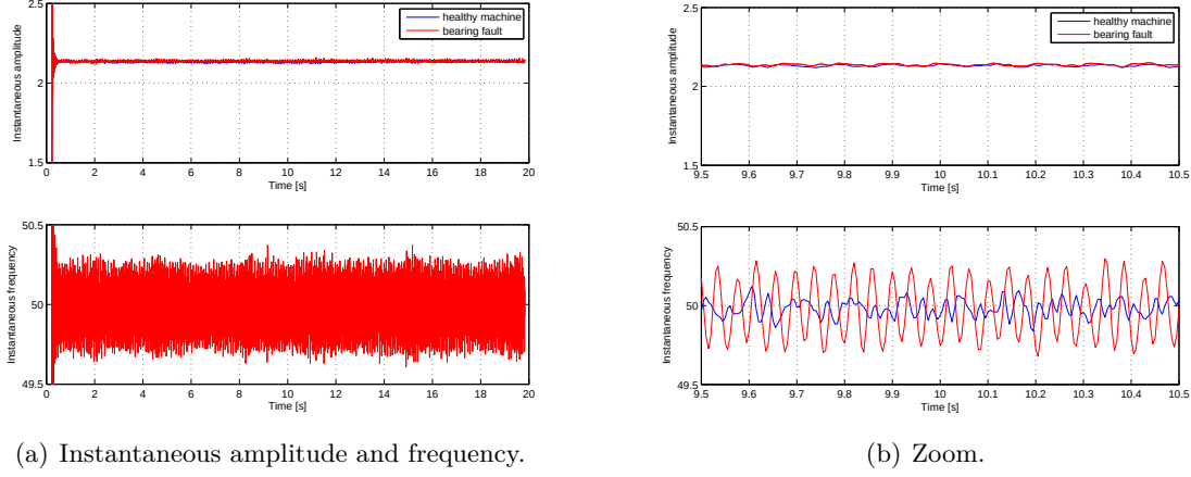
Figure 4.7: Concordia Transform-based demodulation.
