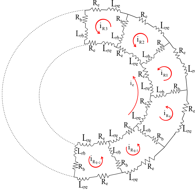
Figure 3.1: Equivalent circuit of a cage rotor showing rotor loop and circulating end-ring current [10].
