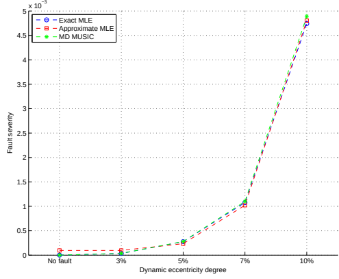
(a) Dynamic eccentricity detection for varying eccentricity degree.
