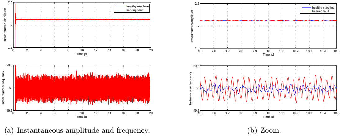
Figure 4.8: Principal Component Analysis-based demodulation.
