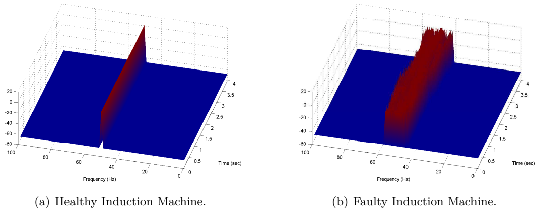
Figure 4.15: Hilbert Huang Transform for a) healthy and b) faulty induction machine.
