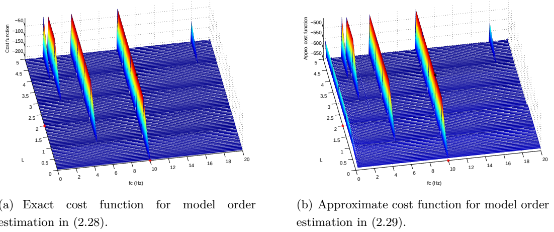
Figure 2.7: Exact and approximate PSD ( f_s = 50\text{Hz} , f_c = 10\text{Hz} and L = 2 )).
