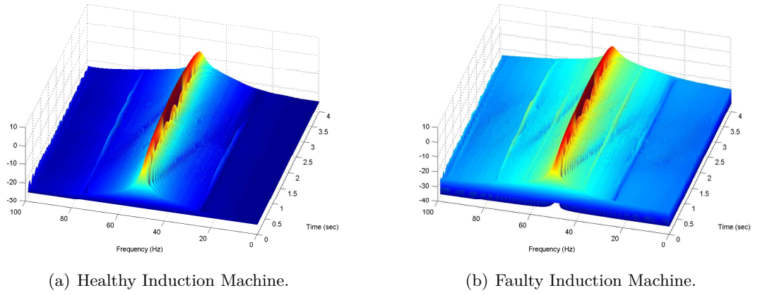
Figure 4.14: Wigner-Ville Distribution for a) healthy and b) faulty induction machine.
