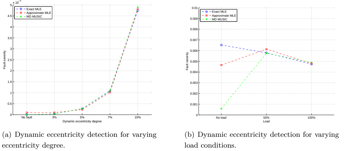
Figure 3.15: Fault detection criterion based on the three methods for dynamic eccentricity detection.
