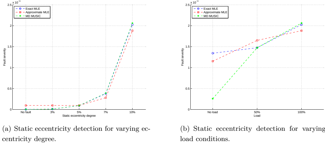
Figure 3.14: Fault detection criterion based on the three methods for static eccentricity detection.
