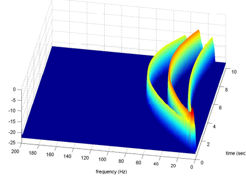
(b) ZAM WV distribution of sinusoidal FM signals with Hanning smoothing window.
