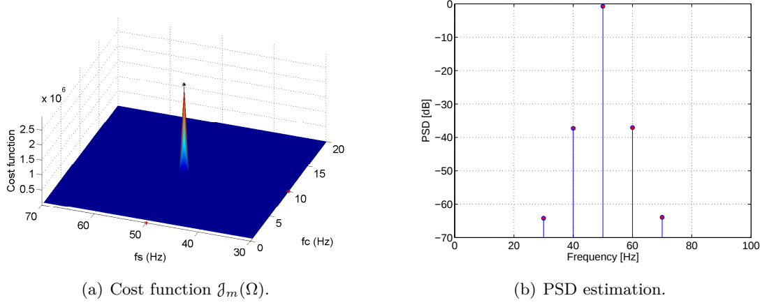
Figure 2.11: Multidimensional MUSIC for the estimation of f_s and f_c .
