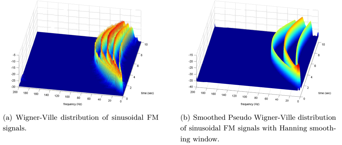
Figure 1.20: Time-frequency representation of sinusoidal FM signals using WVD.
