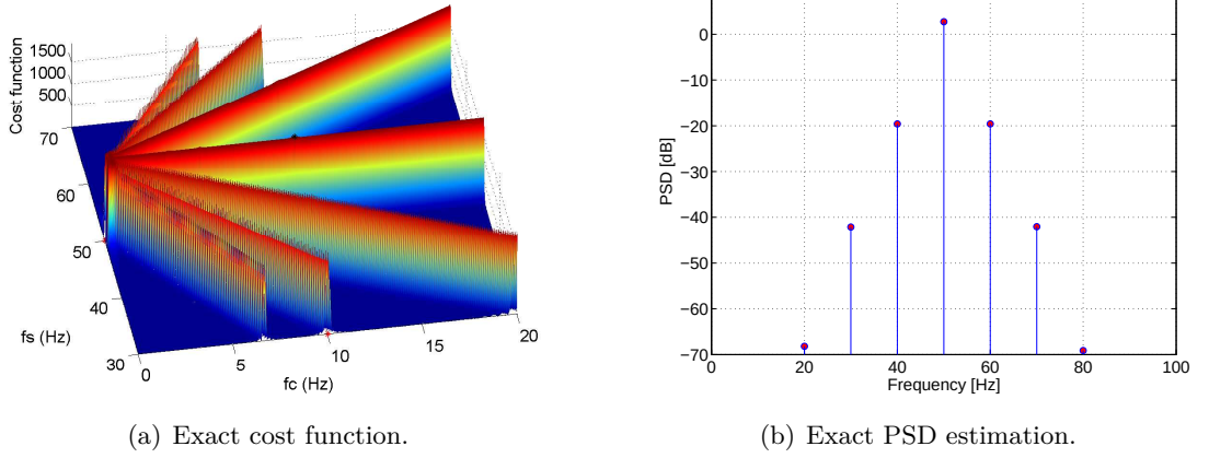
Figure 2.5: Exact cost function \mathcal{J}(\Omega) and signal PSD ( f_s = 50\text{Hz} , f_c = 10\text{Hz} and L = 2 ) for a wrong value of model order.
