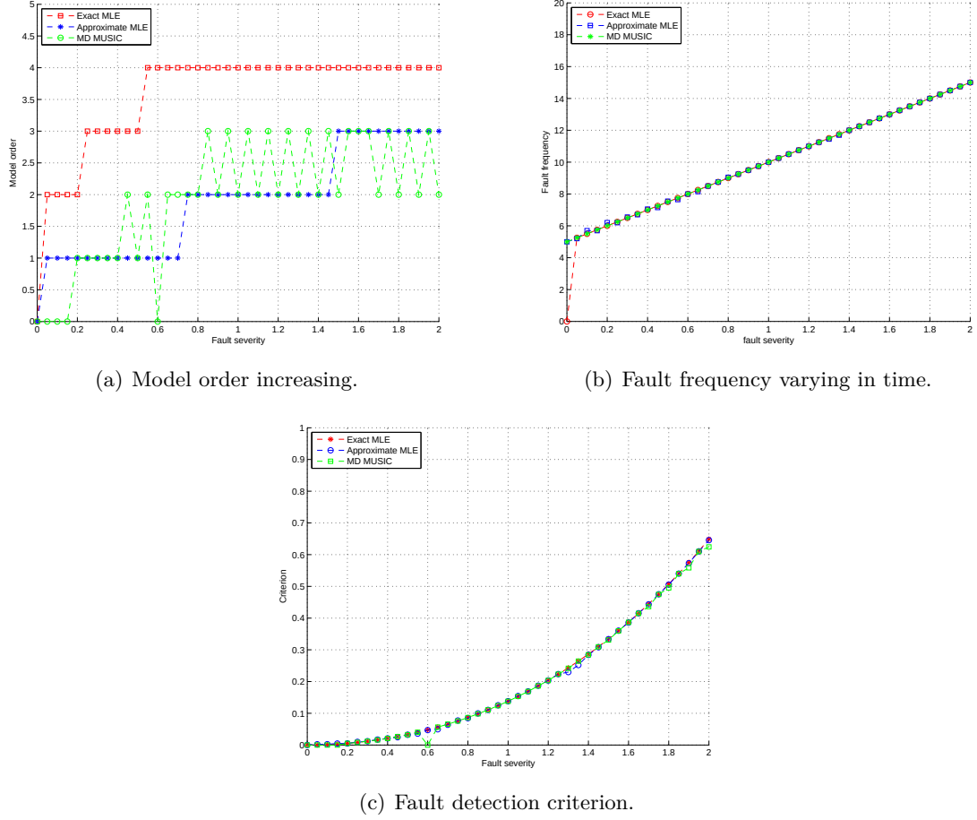
Figure 2.18: MLE-based L , f_c , and criterion \mathcal{C}(n) for fault severity increasing.
