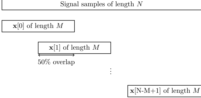
Figure 2.9: Signal segmentation.
