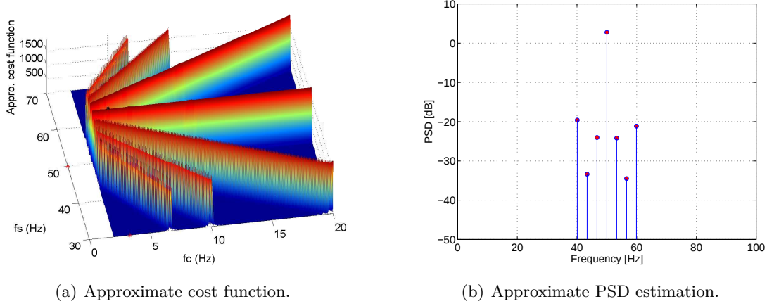
Figure 2.6: Approximate cost function \mathcal{J}_a(\Omega) and signal PSD ( f_s = 50\text{Hz} , f_c = 10\text{Hz} and L = 2 ) for a wrong value of model order.
