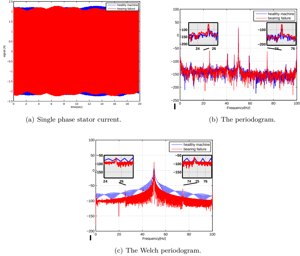
Figure 4.4: PSD of stator current with bearing fault vs. healthy case.
