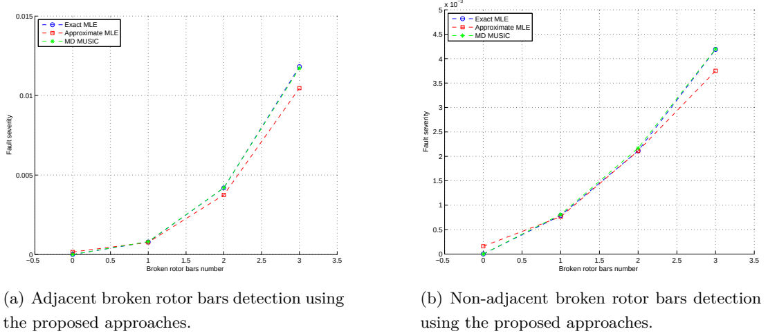
Figure 3.7: Fault detection criterion based on the three methods for broken rotor bars detection: fault severity increasing.
