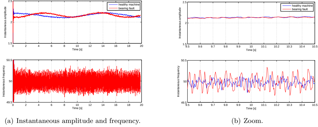
Figure 4.10: Teager energy operator-based demodulation.
