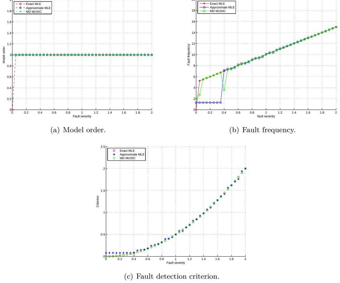
Figure 2.17: Proposed approaches on synthetic signal: L , f_c , and criterion \mathcal{C}(n) estimation for fault severity increasing.
