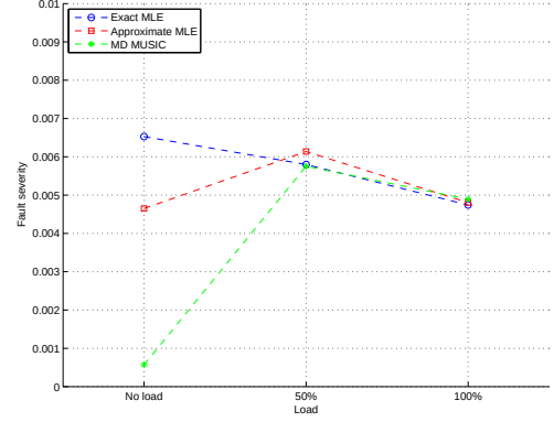
(b) Dynamic eccentricity detection for varying load conditions.
