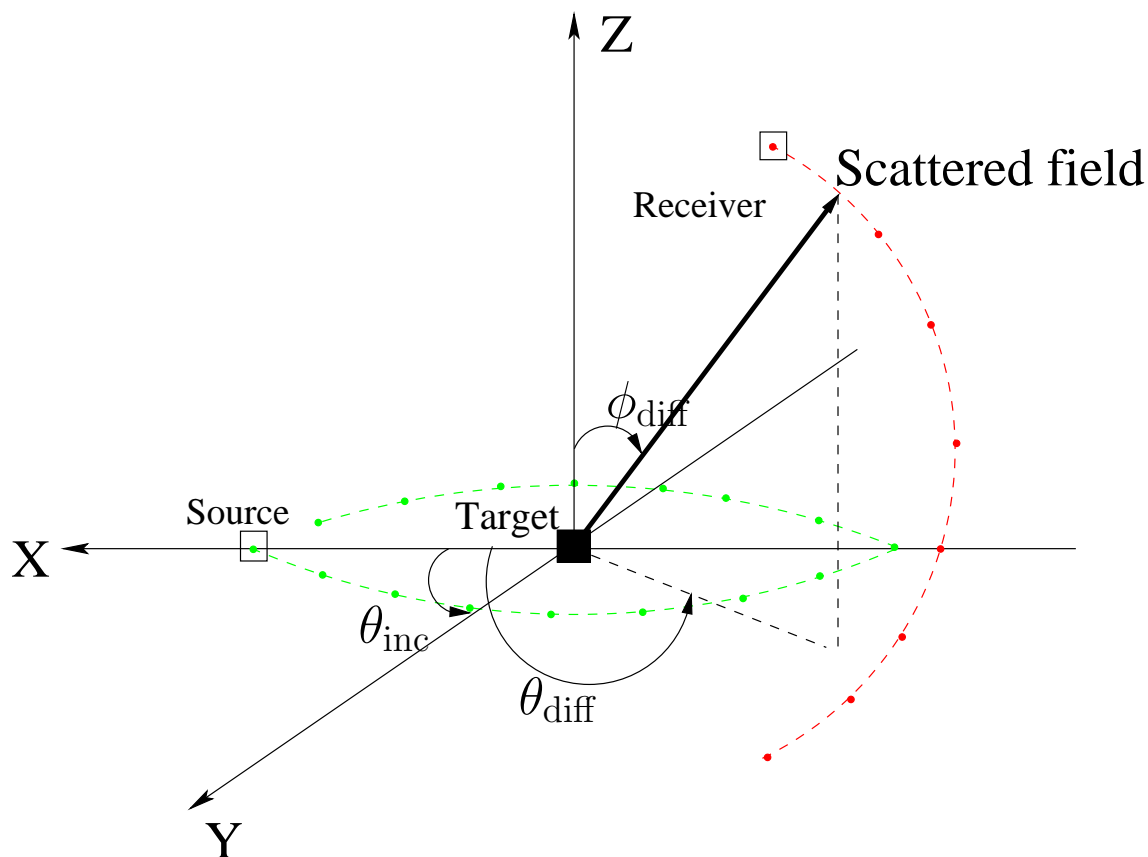
Figure 7.1 : Sketch of the experimental setup. The illumination is done on the (x, y) plane with \theta_{\text{inc}} ranging from 0^\circ to 350^\circ with a step 10^\circ (green line). The receiver position \theta_{\text{diff}} ranges from 0^\circ to 320^\circ with the angular step 40^\circ and \phi_{\text{diff}} ranges from 30^\circ to 150^\circ with the step 15^\circ (red line).
