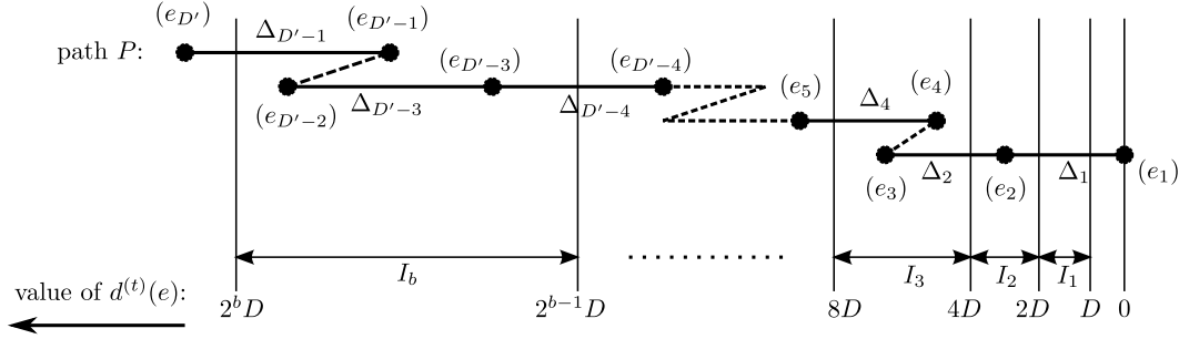
FIGURE 3.1: An illustration of sets I_i and \Delta_i in the proof of Theorem 3.6.
