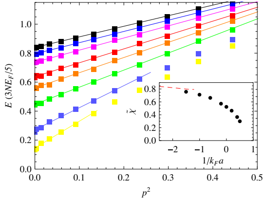
FIG. 1 (color online). Canonical equation of state of a two-component Fermi gas calculated using quantum Monte Carlo simulation, for 1/k_F a = -1.5, -1, -0.6, -0.2, 0, 0.2, 0.4, 0.5 (from top to bottom). The solid lines are fits of the low-polarization data with Eq. (2). Inset: Extracted values of the susceptibility \tilde{\chi} as a function of 1/k_F a . The dashed red line is the result of a perturbation expansion valid up to order (k_F a)^2 .
