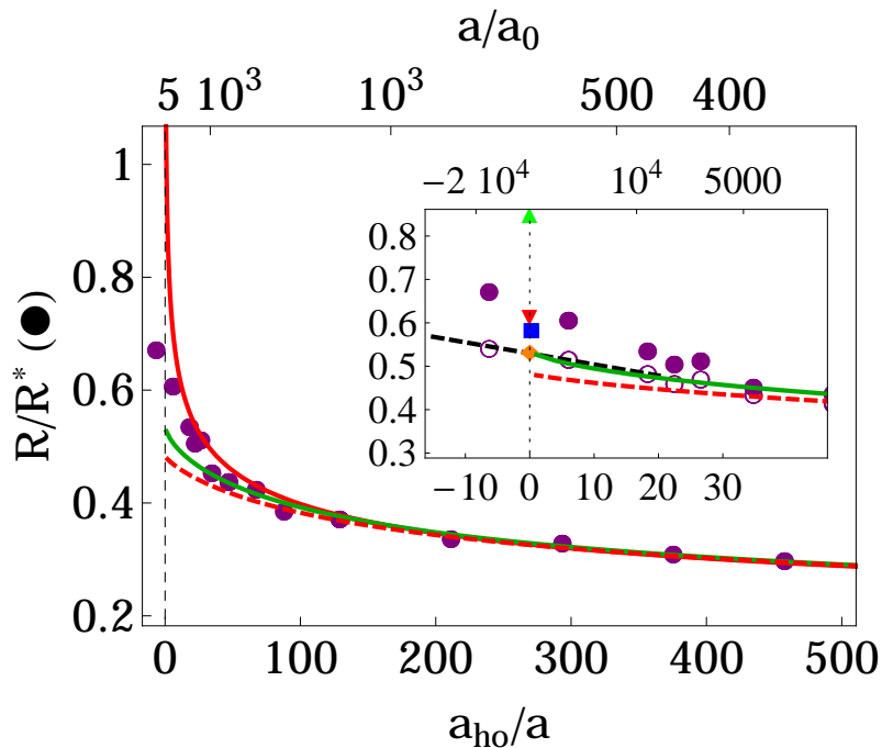
Figure 4.7: Normalized cloud radius R/R^* (filled purple circles) as a function of the inverse scattering length a_{\text{ho}}/a at the end of a 75-ms magnetic-field sweep. The static mean-field prediction is plotted in solid red line, the mean-field scaling solution in dashed red, and the beyond mean-field scaling ansatz in solid green line. Inset: Zoom around the unitary limit. Predictions for the universal constant \xi_B are shown in up green up triangle [55], red down triangle [56], blue square [57], and orange diamond [58]. The filled (empty) circles correspond to the radii normalized to the final (initial) atom number. The dotted black line is a linear interpolation at unitarity (see text).
