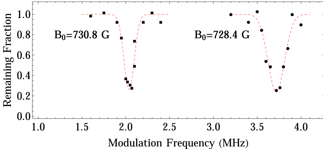
Figure 3.5: Radio-frequency association spectra of {}^7\text{Li}_2 molecules taken at magnetic fields of 728.4 G (circles) and 730.8 G (squares).
