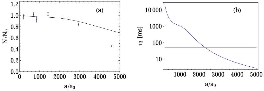
Figure 4.4: (a): Atom number measured after a sweep time of 150 ms, where N_0 = 3.8 \cdot 10^4 as a function of the final scattering length a/a_0 . Each experimental point is an average of about 10 shots. The black solid line is a simple model for the atomic losses in quasi-equilibrium conditions. (b): Three-body recombination time \tau_3 as a function of the scattering length a/a_0 . The red solid line is the axial trapping period of 54 ms.
