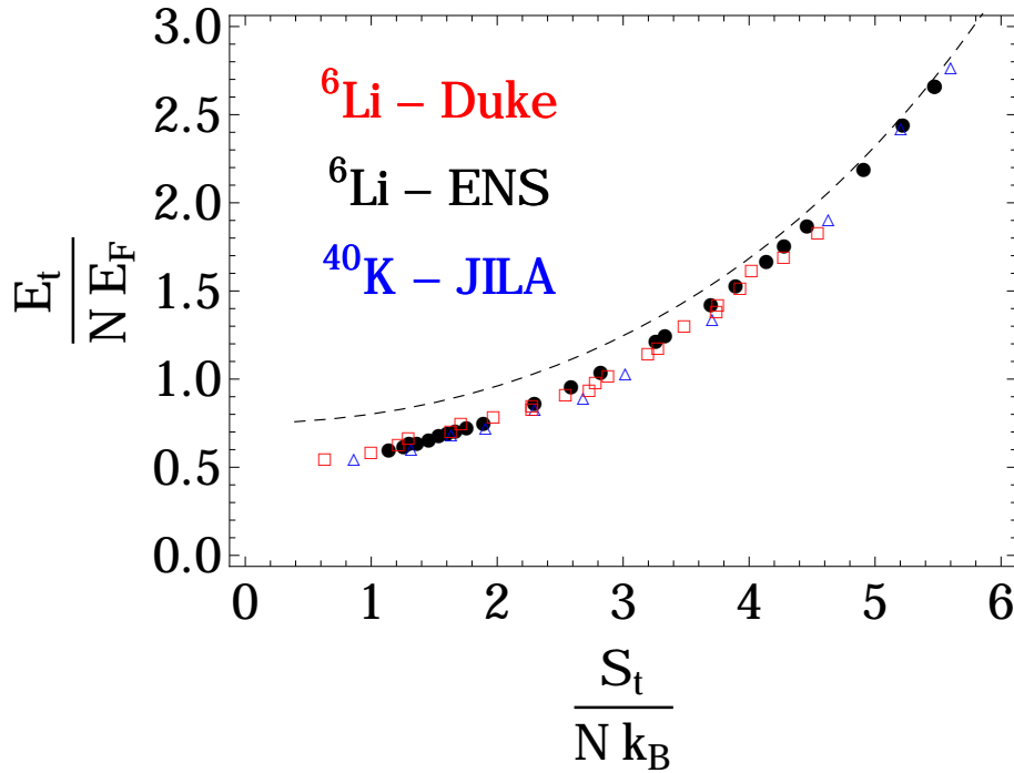
Figure 5.15: Universality of the unitary Fermi gas: the equation of state in the canonical ensemble for the trapped gas. The energy E_t/N E_F is plotted versus the entropy per particle S_t/N k_B . The data from Duke University on {}^6\text{Li} (red squares, [249]) and JILA on {}^{40}\text{K} (blue triangles, [108]) are plotted together with the EoS deduced from our measurement on {}^6\text{Li} of the homogeneous EoS (black dots). The ideal gas EoS is shown in dashed black line.
