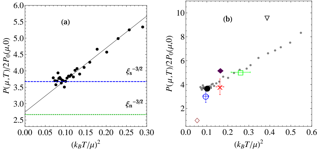
Figure 5.14: Normal/superfluid phase transition in the unitary Fermi gas. (a): Low-temperature deviation to the Fermi liquid behavior. The T = 0 compressibility of the superfluid (normal fluid) \xi_s ( \xi_n ) is shown in dashed blue line (dotted green line). (b): Comparison between the experimental critical point (black dot) and theoretical predictions: 1/N expansion (brown diamond [240]), Diagrammatic Monte-Carlo calculations from Burovski et. al. (blue circle [241]) and Gouliko et. al. (red cross [242]), Quantum Monte Carlo (green square [230]), self-consistent diagrammatic approach (solid purple diamond [202]), a Borel-Padé approximation connecting a \epsilon -expansion (black down triangle [243]) (the result for the \epsilon = 1 of the \epsilon = 4 - d expansion is off range [243]).
