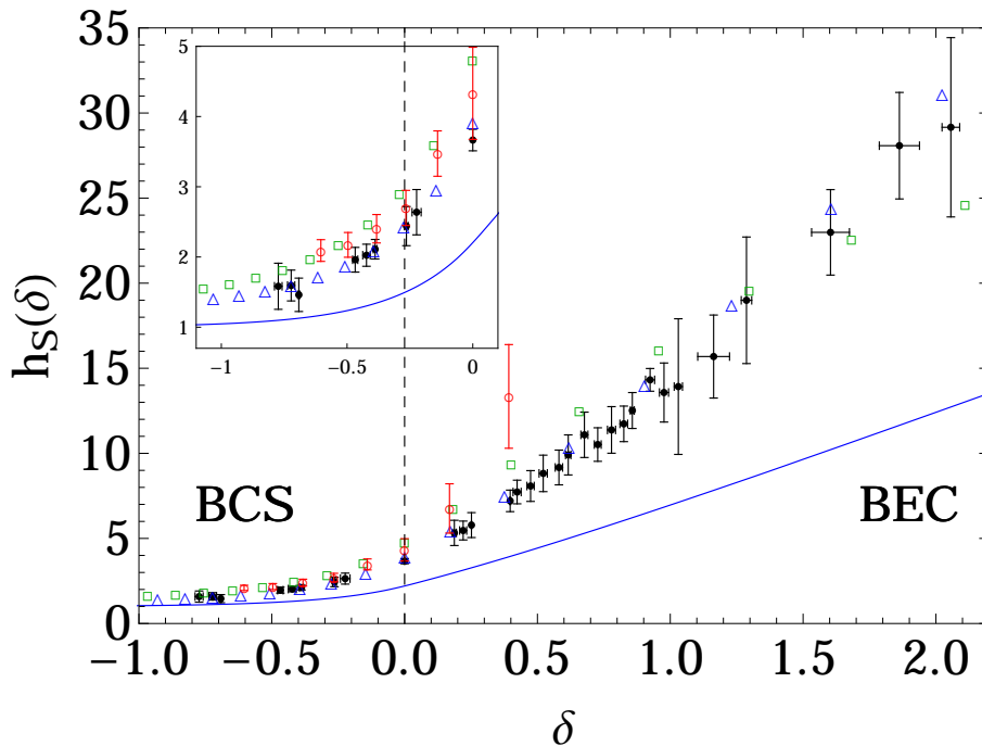
Figure 5.18: Equation of state of a low-temperature Fermi gas in the BEC-BCS crossover. The experimental data (black dots) are compared to different zero-temperature theories: a Quantum Monte Carlo calculation (red circles [230]), a self-consistent t-matrix approach (green squares [202]), a Nozières-Schmitt Rink approximation (blue triangles [259]), and the BCS-mean-field theory (blue solid line [21,22]). Inset: Zoom on the BCS side of the resonance ( \delta < 0 ).
