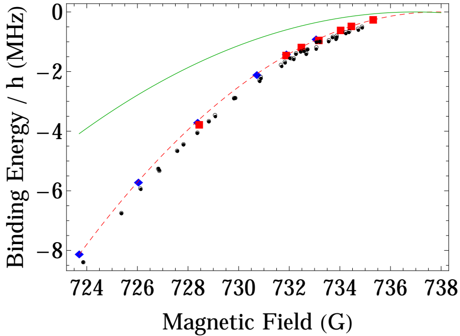
Figure 3.6: Binding energy of {}^7\text{Li}_2 Feshbach molecules. The final magnetic field is ramped with the Feshbach coils (blue diamond) or the Offset coils (red squares). The dashed red line is a parabolic fit of the data to the universal law Eq.(3.12) from which the scattering length is deduced. In black dots the Bar-Ilan measurement [79], in solid green line the binding energy deduced from the Feshbach resonance measurement of the Rice group [155].
