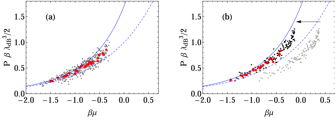
Figure 5.2: Determination of the global chemical potential \mu_0 on a finite-temperature unitary Fermi gas. The normalized pressure P\beta\lambda_{\text{dB}}^3/2 is plotted against the normalized chemical potential \beta\mu . Each image has \beta\mu_0 as a free parameter, corresponding to a horizontal shift on these plots. (a): The global chemical potential on the high-temperature images (grey points) is fitted using the second-order virial coefficient (solid blue line) rather than the classical gas (dashed blue line) and the images are averaged to obtain a low noise EoS (red). (b): \mu_0 is adjusted on lower temperature images to minimize the distance in the overlapping region of the EoS determined from the hotter samples.
