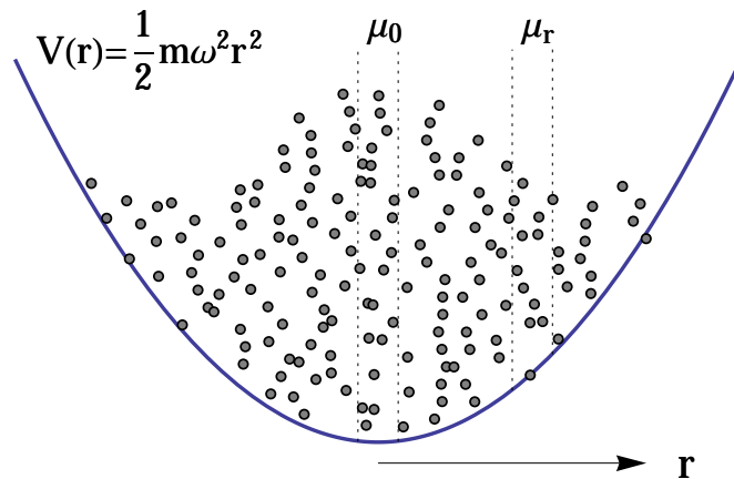
Figure 1.7: Sketch of the local density approximation. The system can be subdivided in mesoscopic volumes (dotted vertical lines) where the system has the properties of the homogeneous gas with a local chemical potential \mu_r = \mu_0 - V(r) , where \mu_0 is the global chemical potential and V(r) the trapping potential (blue solid line).
