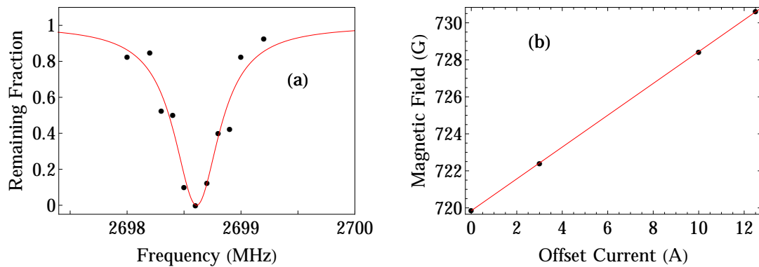
Figure 2.11: Calibration of the magnetic field using {}^7\text{Li} . (a): Remaining atoms in |1\rangle after 50 ms of radio-frequency at a magnetic field of 730.6 G. (b): Magnetic field (determined by the position of the maximum of loss) as a function of the current in the Offset coils (with 361 A in the Feshbach coils, and 45 A in the curvature coils).
