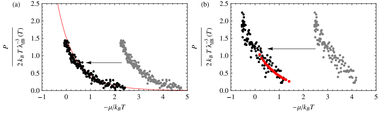
Figure 2. Determination of \mu^0 : we plot the data from an in situ image as P/2k_B T \lambda_{\text{dB}}^{-3} versus -\mu/k_B T = V(z)/k_B T - \mu^0/k_B T (black points). A wrong choice of \mu^0 in this representation corresponds to a translation of the data in abscissa. We adjust \mu^0 so that the wings of the pressure profile match a reference equation of state (in red). (a) For high-temperature clouds, we use the second-order virial expansion (3). (b) For a lower temperature pressure profile, we minimize its distance with the averaged equation of state deduced from higher temperature images (in red) in the overlap region.
