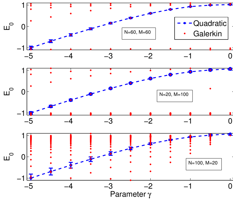
Figure 4.3: The graph captures the evolution of E_0 as it crosses the spectral gap of H_{-1} where \phi_{\text{el}}(r) = \gamma/(1 + r^2) for \gamma = -5 : .5 : 0 . We consider three choices of pairs (N, M) such that \dim(\mathcal{L}_{NM}) = 120 . The curve corresponds to \Re(\lambda_n) for \lambda = \lambda_n in (4.8) and (4.10). The vertical bars on the curve measure |\Im(\lambda_n)| . We superimpose the image with the eigenvalues of L in (4.6) for G = H_{-1} , that is the Galerkin approximation.
